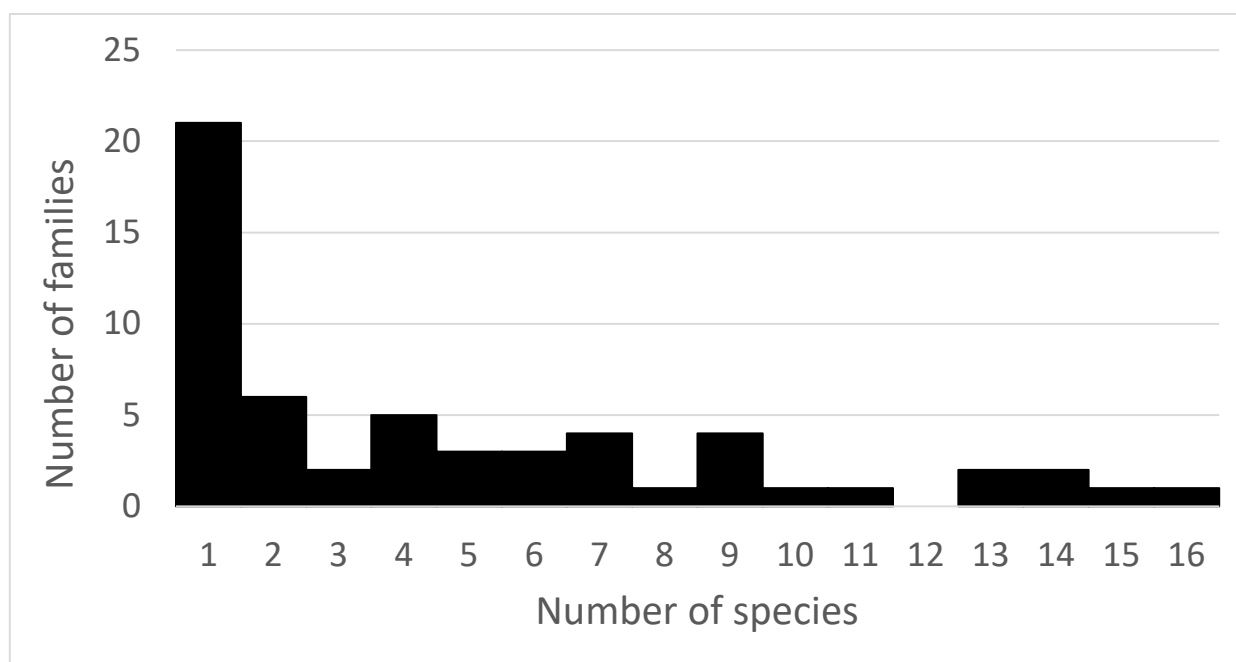
Figure 2. Distribution of the numbers of species belonging to the 57 amphipod families recorded in the English Channel.
