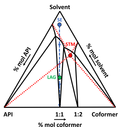
Figure 13. Schematic isothermal ternary phase diagram describing a system forming a 1:1 and a 1:2 cocrystal with congruent solubilities. The red point is the theoretical eutectic composition between API and the coformer at that specific temperature (solution doubly saturated in API and the coformer, computed from pure component ideal solubilities) chosen as the screening composition for the STM method. The green point corresponds to an arbitrary stoichiometric ratio screened by the LAG method. The blue dashed line corresponds to the crystallization pathway with the SE method from a stoichiometric undersaturated solution (blue point).
