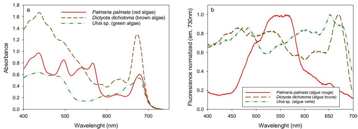
Figure 6. a: Example of spectral absorbance ( A_\lambda ) between 400-700 nm and b: Example of fluorescence excitation spectra between 400-700 nm with an emission measured at 730 nm performed on Chlorophyta (green algae), Rhodophyta (red algae) and Phaeophyceae (brown algae) from the Bay of Cherbourg.
