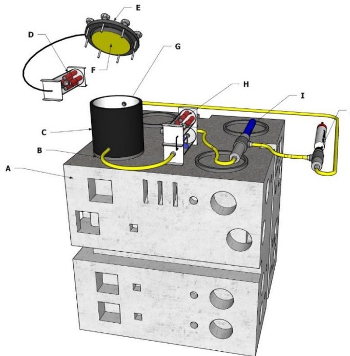
Figure 2. Automated benthic chamber for primary production measurement. (A) MARINEFF eco-engineering dyke module with the mooring ring (B) to fix the benthic chamber (C). Aluminium tape (G) covers the benthic chamber inside. LED panel (F) is fixed to the benthic chamber top (E) which is screwed on the benthic chamber to close it hermetically. The LED panel is driven by the LED controller (D). Water flow is generated by an underwater pump (H). Two sensors, YSI EXO 1 (I) with oxygen probe, and Turner Design C-Sense pCO 2 probe (J) driven by the RBR Virtuoso3 logger (J), measures the gas concentration. The whole system is in a water closed circuit connected by pipe.
