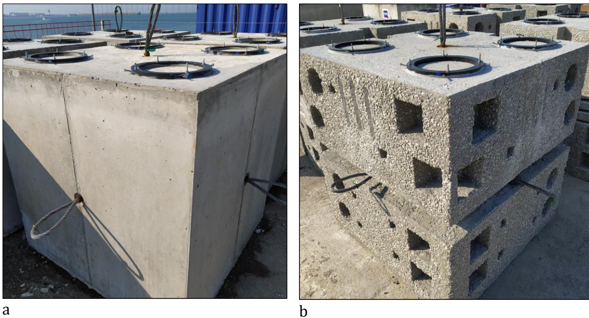
Figure 1. Dyke modules deployed during the MARINEFF project: a: classic module; b: Eco-engineering module.
