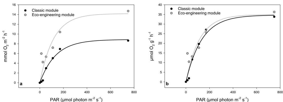
Figure 5. Example of Production / Light curves measured on MARINEFF eco-engineering dyke module and classic dyke module in the Bay of Cherbourg in April 2021. Dots show the GPP measurements at each light intensity (PAR) and the lines show the Webb model fits. a: GPP expressed as a function of subtract surface and time; b: GPP expressed as a function of fresh weight of macroalgae and time.
