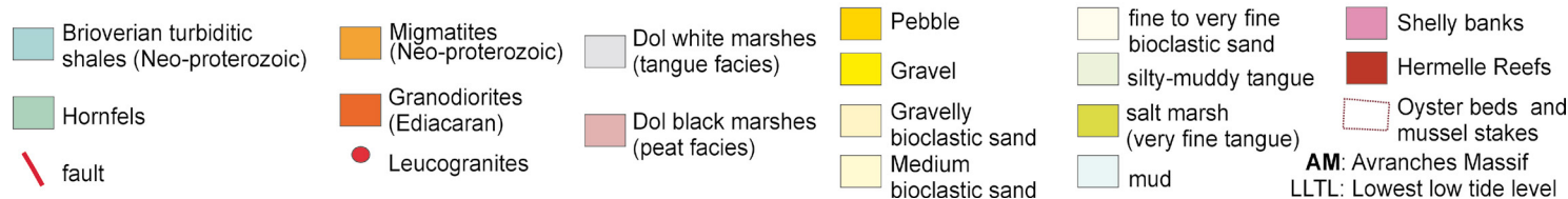
Fig. 2 - Simplified geological and sedimentological map of the Mont-Saint-Michel bay (after Larsonneur, 1989; L'Homer et al., 1999a).
