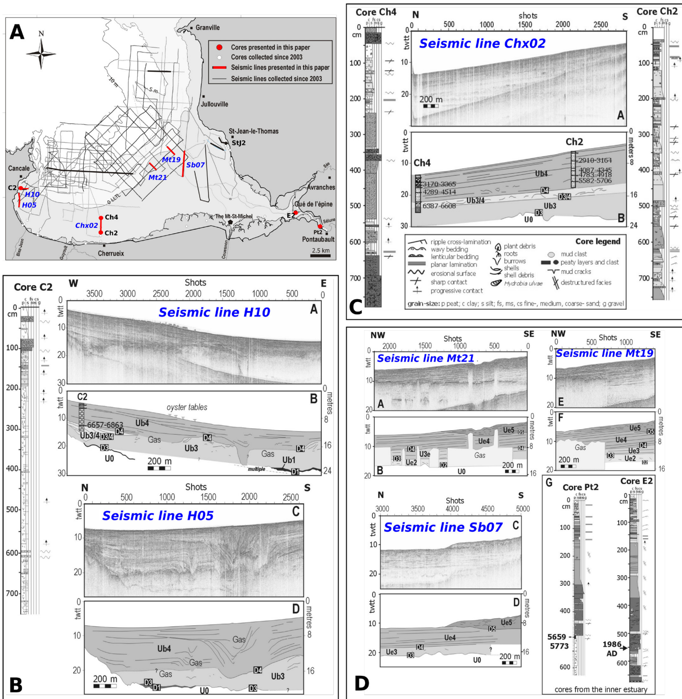
Fig. 19 - Examples of very high-resolution seismic lines (raw and interpreted) and vibrocores acquired in the MSMB. A) Location map of the data (Lines and cores on B, C, D are indicated in red). B) From the mudflat in the embayment - Cancale Bay. C) From the sandflat in the embayment - Cherrueix. D) From the external (seismic lines) and internal (cores) estuary. Data from Billeaud (2007), figures in Tessier et al. (2010). All ages are in Cal. yr. BP. Uxn: Seismic Units and Dx: discontinuities as defined in Billeaud (2007) and Tessier et al. (2010).
