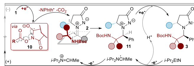
♦ Inhibition reaction: + TEMPO (3 equiv) → traces of 3fa (conditions of Table 1, entry 1) ♦ Cyclic Voltammetry experiments (V vs SCE in DMF): 1a , E = -1.25 V; 1f , E = -1.27 V, 2a , E red = -1.66 V and E ox = +1.56 V; 3af , E ox = +1.12 V and +1.56 V; i -Pr 2 EtN, E = +0.88 V
