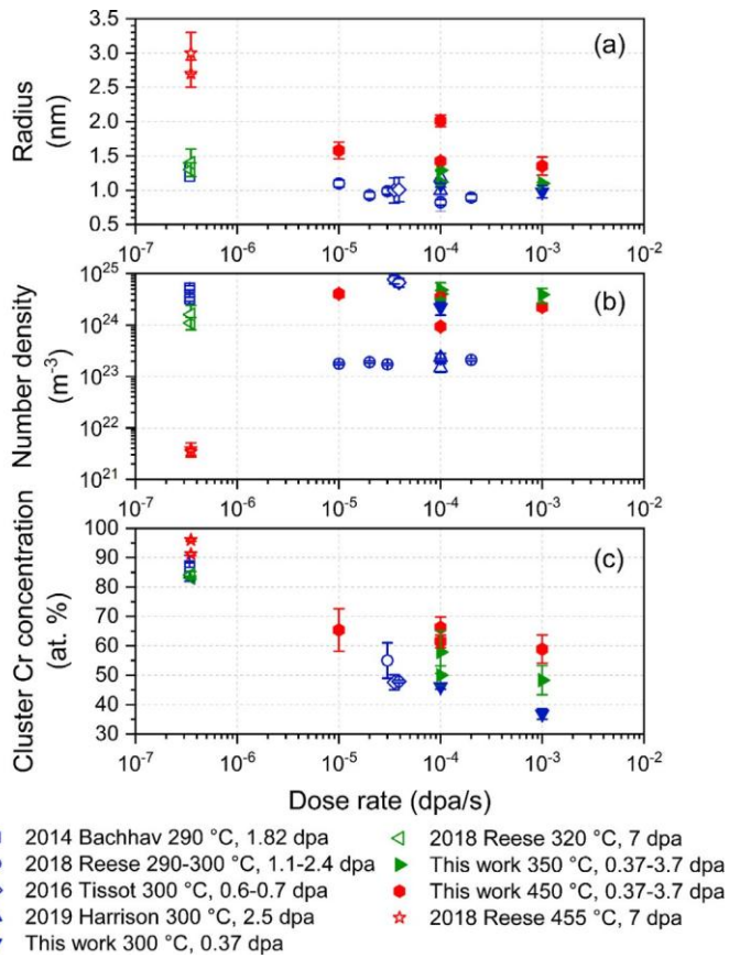
Fig. 10. Comparison of (a) radius, (b) number density and (c) Cr concentration of CrRP in Fe(15–19)Cr after ion ( 10^{-5} to 10^{-3} dpa/s) and neutron ( \sim 3 \times 10^{-7} dpa/s) irradiation up to 7 dpa. The
