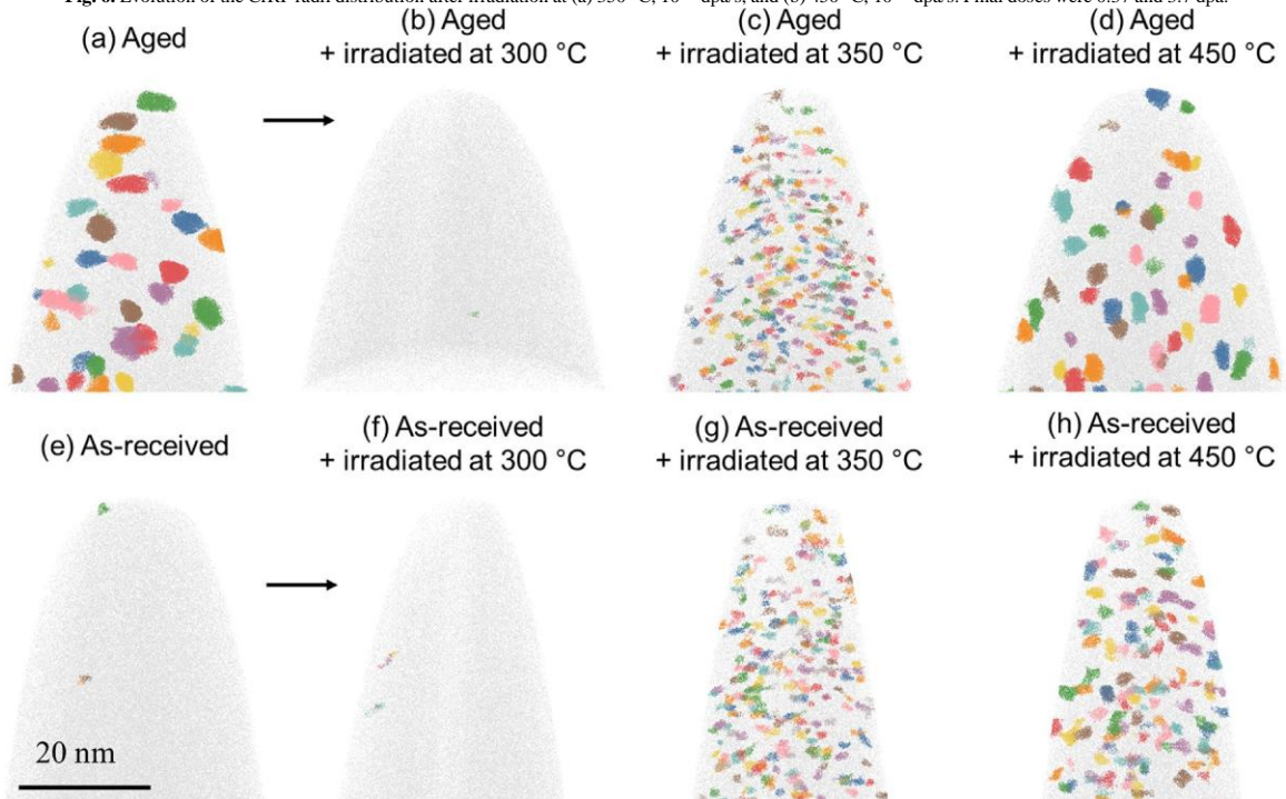
Fig. 7. APT reconstructions showing CrRP evolution in Fe-18Cr. (a) Sample aged at 500 °C for 900 h. Samples aged at 500 °C for 900 h followed by ion irradiation at (b) 300 °C, (c) 350 °C and (d) 450 °C. (e) Unirradiated as-received material. Samples that were ion irradiated from the as-received state at (f) 300 °C, (g) 350 °C and (h) 450 °C. The dose rates and doses were 10^{-3} dpa/s and 0.37 dpa for all the irradiated specimens.
