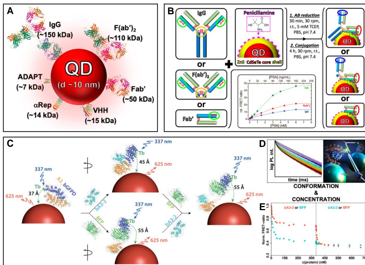
Figure 4. Size and orientation of QD-antibody conjugates. (A) Schematic presentation of biological recognition proteins with various sizes attached to QD surfaces. Protein structures adapted from the RCSB Protein Data Bank (rcsb.org) PDB IDs “1TGT” (for IgG, F(ab) 2 , and Fab’), “5IVO” (for VHH), “3LTJ” (αRep), and “1GJT” (ADAPT). (B) Mild reduction of antibody disulfides (green and orange circles) for direct conjugation to QDs. The different orientations result in surface-near and surface-far antigen binding sites (red and blue circles). The smaller the antibody, the better the immunoassay detection performance (assay calibration curve in the center). Adapted with permission from ref. 49. Copyright 2016 The Royal Society of Chemistry. (C) An αRep bidomain (A3_gGFPD) with a Tb donor and QD acceptor leads to Tb-to-QD FRET upon Tb excitation. Depending on target binding of bA3-2 (top), BFP (bottom), or both (right), the bidomain conformation changes. (D) PL decay time analysis can quantify the conformational changes shown in C. (E) TG-FRET ratios of QD and Tb PL can quantify the target concentrations during sequential target-bidomain binding. C to E reproduced with permission from ref. 1. Copyright 2020 American Chemical Society.
