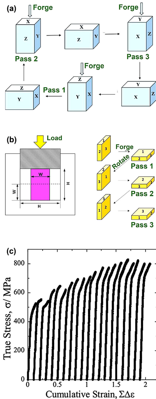
Figure 17. (a) Principles of the multi-directional forging method [226]. (b) Principles of the cyclic closed die forging method [228]. (c) Stress-strain curves for titanium processed by multi-directional forging for 20 passes at room temperature [233].
