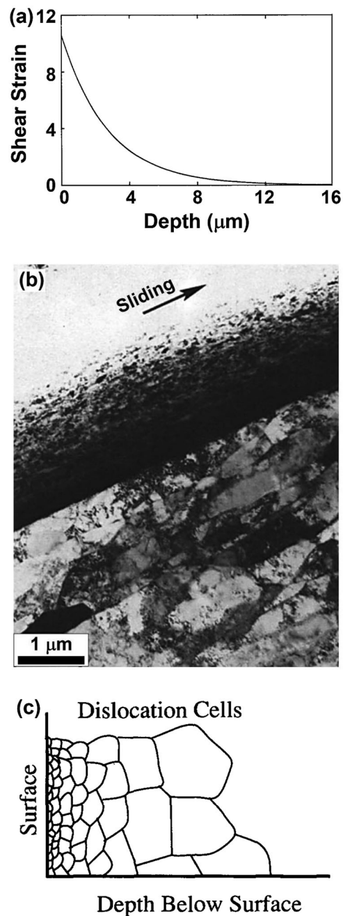
Figure 8. (a) Estimation of surface severe plastic deformation by sliding reported by Rigney et al. [89]. (b) Gradient microstructure in copper processed by sliding [89]. (c) Schematic illustration of gradient microstructure formation in aluminum by sliding [90].
