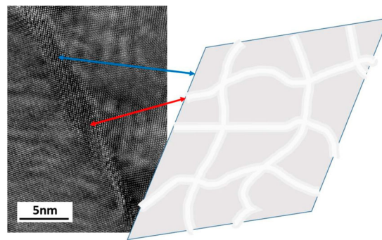
Figure 32. Schematic plane-view of a heterogeneous distribution of the excess free volume in a deformation-modified high-angle grain boundary. The deformation-induced distortion is localized to channels (light gray) where the excess free volume exceeds the values typical for a relaxed high-angle grain boundary. The undistorted (relaxed) regions are colored in gray. Such areas in a high-angle grain boundary of copper processed by equal-channel angular pressing are specified for its cross-section view [628].
