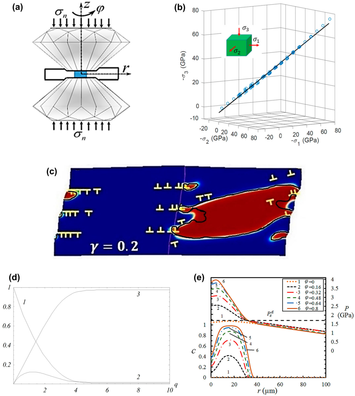
Figure 30. (a) Schematics of shear (rotational) diamond anvil cell, in which a sample within a gasket is compressed and twisted by diamond anvils [566]. (b) The crystal lattice instability criterion in the space of normal-to-cubic-faces stresses ( \sigma_i ) for Si-I \rightarrow Si-II phase transformation obtained within the phase field approach (plane) [607] and confirmed by the first-principles calculation (points) [593]. (c) The high-pressure phase (red) obtained under compression and shear of a bicrystal at the stress concentrators produced by dislocation pileups [595]. (d) Evolution of the volume fraction of Si-I (1), Si-II (2), and Si-III (3) under plastic straining at a pressure of 7 GPa obtained from solution of the theoretical strain-controlled kinetic equation [601]. (e) Distributions of the pressure ( P ) and concentration ( c ) of the \omega phase at the contact surface between a zirconium sample and diamond anvil during twisting under the fixed axial force [604].
