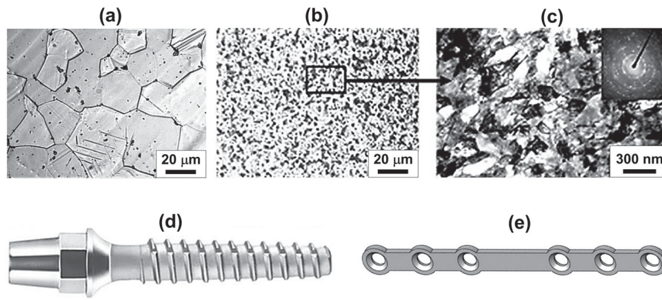
Figure 50. (a-c) Microstructure of commercially pure grade 4 titanium: (a) optical micrograph of initial coarse-grained rod, (b) optical and (c) transmission electron micrograph of nanograined titanium processed by equal-channel angular pressing and thermo-mechanical treatment [955]. (d) Dental implant [960,961] and (e) medical mini-sheet fabricated from nanograined titanium [955,956].
