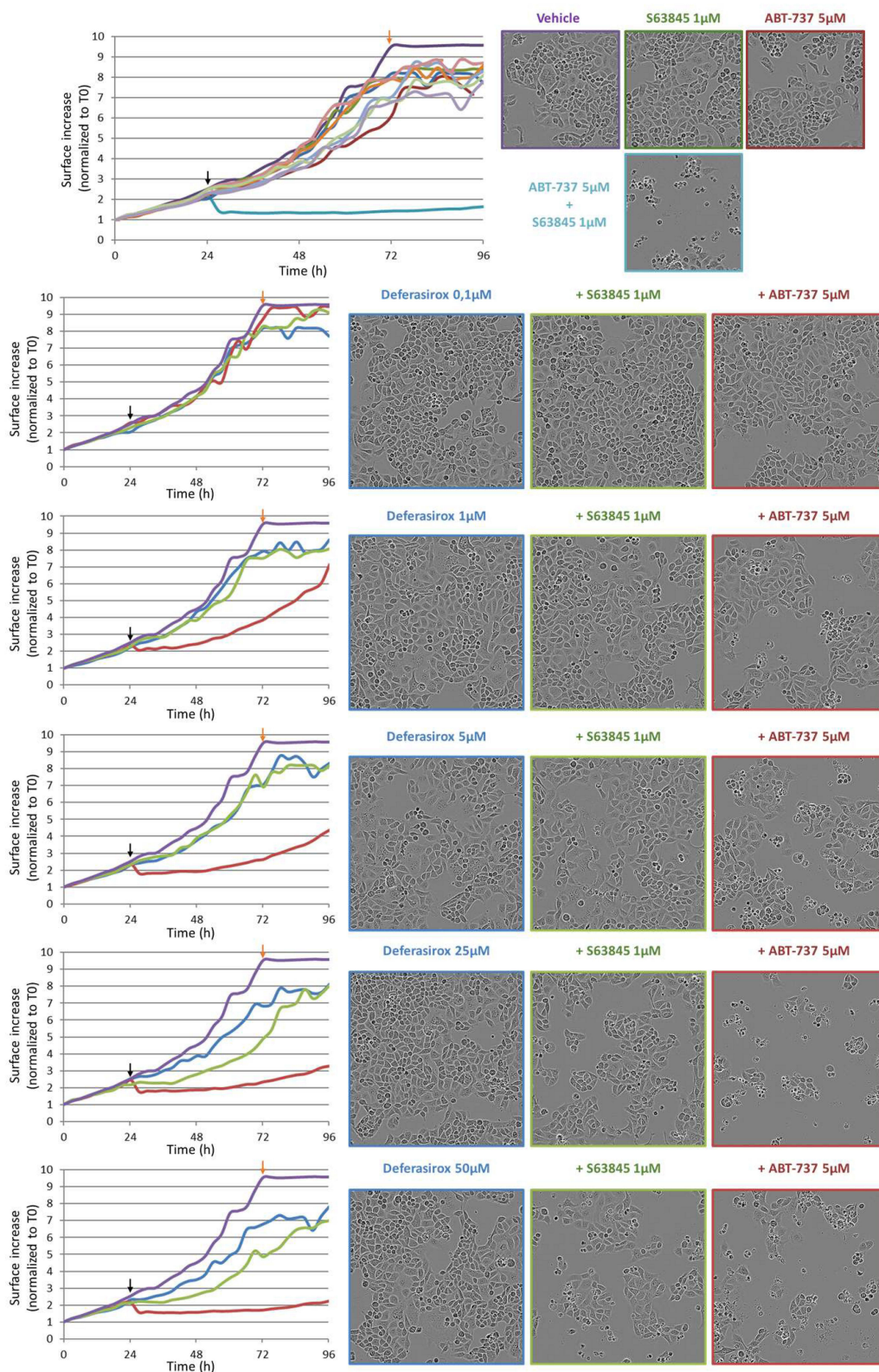
Figure 8 Time and concentration effect of Deferasirox combined with ABT-737 5µM or S63845 1µM on IGROV1-R10 cell line. Black arrows correspond to treatment time and Orange arrows highlight the 48h exposure time, corresponding to photos.
