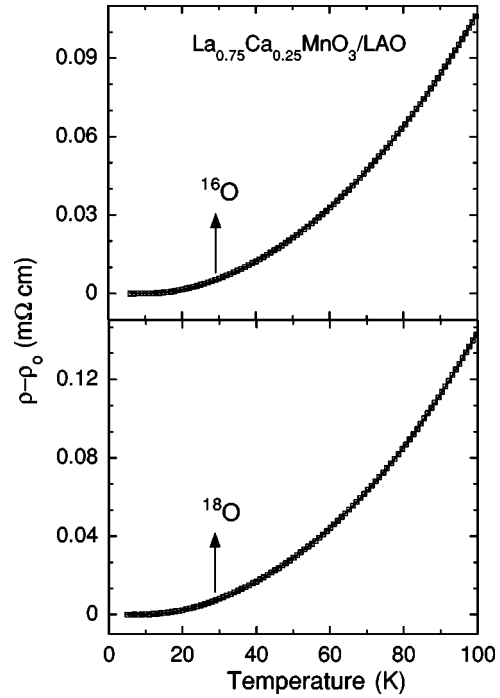
FIG. 3. \rho(T) - \rho_o for the ^{16}\text{O} and ^{18}\text{O} films of \text{La}_{0.75}\text{Ca}_{0.25}\text{MnO}_3 . The solid lines are fitted curves by Eq. (1).
