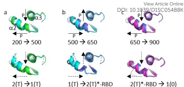
Fig. 4 Structural differences in the segment Ala 59 – Val 109. (a) (Top) Ras(wt) structures at 200 MPa (green) and at 500 MPa (cyan) (Bottom) 3tgp (green) and 5b30 (cyan). (b) (Top) Ras(wt) structures at 500 MPa (cyan) and at 650 MPa (slate) (Bottom) 5b30 (cyan) and 1nvv chain Q (slate). (c) (Top) Ras(wt) structure at 650 MPa (slate) and Ras(D33K) structure at 900 MPa (pink) (Bottom) Ras bound to the regulatory (slate) and catalytic (pink) sites in the ternary complex Ras(Y64A).GppNp:SOS:Ras(wt) ( 1nvv chain Q and chain R). Solid arrows show the direction of displacement when pressure increases, and dashed arrows show the direction of displacement from one state to another.
