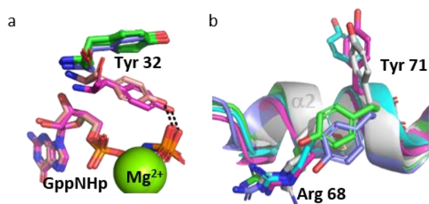
Fig. 6 (a) Tyr 32 and GppNHp in stick representation in Ras(wt) at 650 MPa (slate) and 900 MPa (pink), in 3tpg (green) and 3oiu (salmon). (b) Cartoon representation of segment Gln 61 – Thr 74 with residue Arg 68 and Tyr 71 in stick representation in Ras(wt) at 0.1 MPa (white), at 200 MPa (green), at 500 MPa (cyan), at 650 MPa (slate) and Ras(D33K) at 900 MPa (pink).
