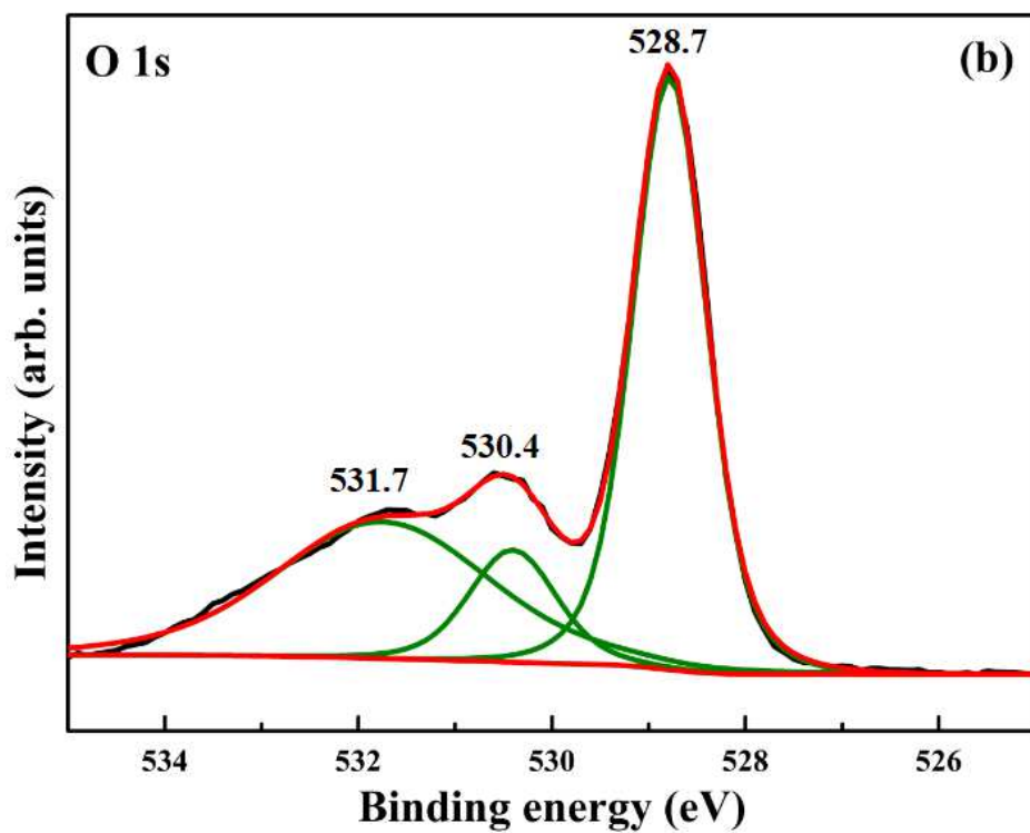
Figure 3. Core level XPS spectra of (a) Ni 2p 3/2 and (b) O 1s of undoped NiO nanoparticles.
