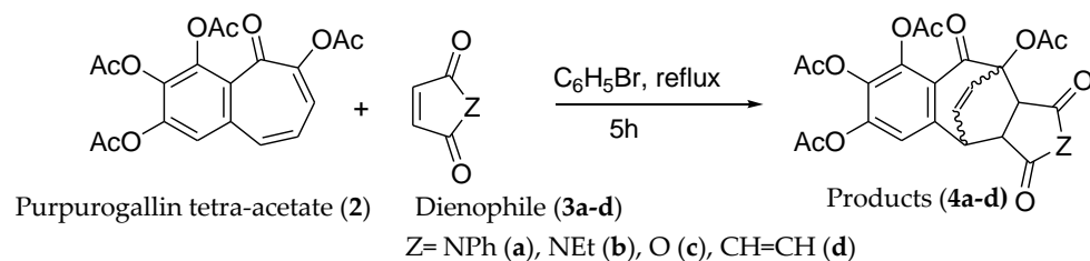
Scheme 2. Diels-Alder reactions between Purpurogallin tetraacetate and various dienophiles ( 3a-d ).
