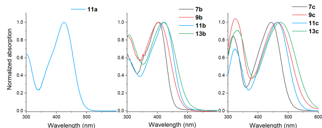
Figure 2. Absorption of triphenylamines in water sorted by pyridinium substitution, ortho compounds (left), meta compounds (middle), para compounds (right).
