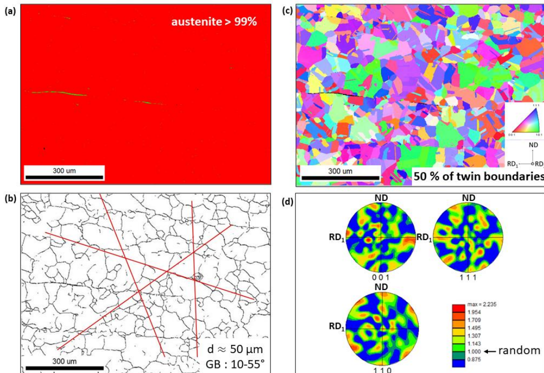
Fig. S1. SEM-EBSD (a) Phase map (red: austenite, green: delta ferrite), (b) random high-angle grain boundary map (excluding coincident site lattice boundaries and low-angle boundaries) with red lines drawn for grain size measurement by the intercept method, (c) orientation map (i.e. inverse pole figure map) and (d) pole figures along low-index directions: [001], [111] and [110].
