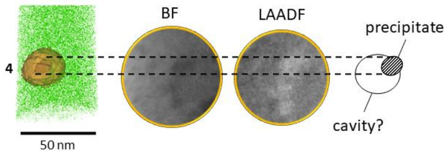
Fig. 13. (Color online) Close-up view of the feature #4 in the STEM LAADF image oriented at \mathbf{B}=\langle 011 \rangle (Fig. 8) and the scheme of suspected defects.
