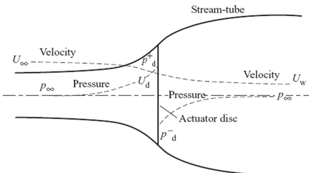
Figure 2: Energy extracting actuator disk and stream-tube.
