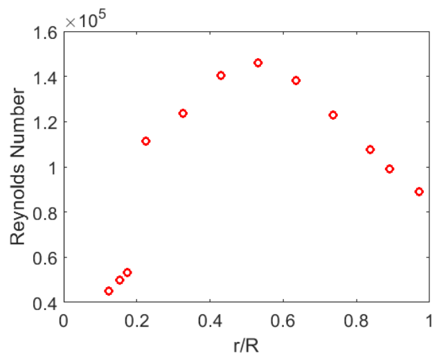
Figure 6: Reynolds Number across the ATIR blade length at flow speed of 1.0m/s at optimum rotational speed of 18.5Hz.
