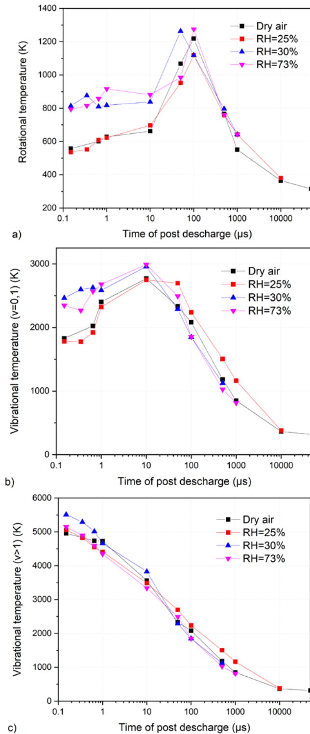
Figure 5: Temporal evolution of the rotational temperature of \text{N}_2(\text{X}) a), the vibrational temperature of v=0,1 b) and the vibrational temperature of v>1 c) during the post-discharge at 85 kV (channel 1) for different relative humidity at 1.5 mm from the pin.
