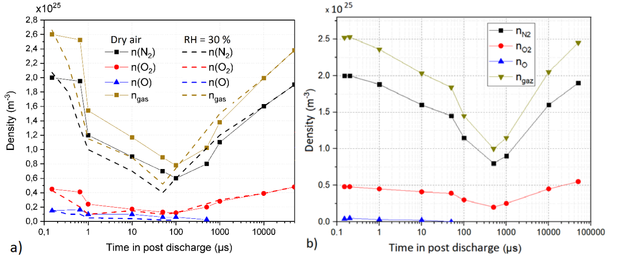
Figure 9: Temporal evolution of the densities of N 2 , O 2 and O for a pulse of 85 kV (channel 1) at 1.5 mm in dry and ambient air a) and at 2.5 mm in dry air b).
