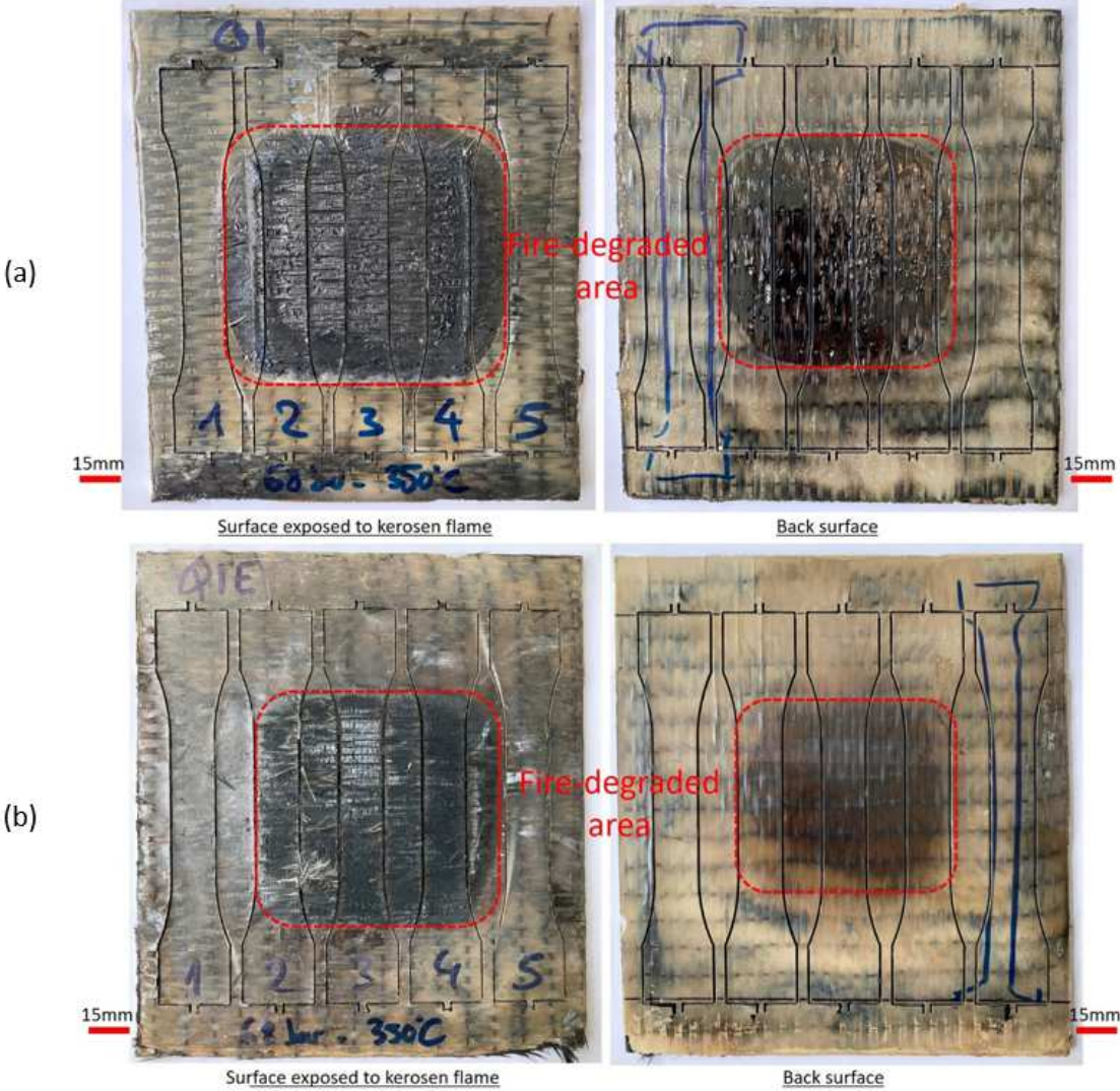
Fig. 9 – Macroscopic observations of quasi-isotropic laminates front and back surfaces: (a) without exolit (PQI) – (b) with exolit (PQIE)
