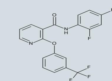
Figure 5 : Diflufenican
