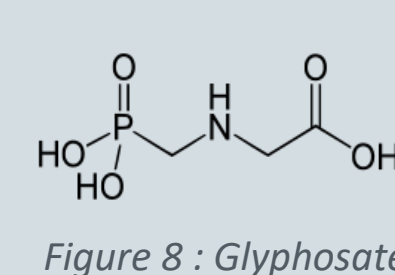
Figure 8 : Glyphosate
