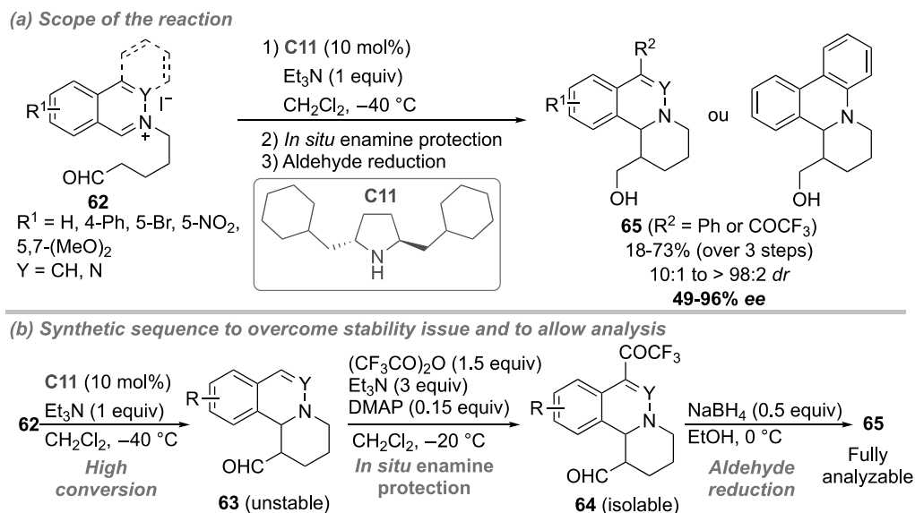
Scheme 18. Diastereo- and enantioselective annulation reaction for the dearomatization of isoquinolinium salts 62 catalyzed by aminocatalyst C11 .
