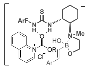
Scheme 12. Addition of boronic acids 36 to quinolinium salts catalyzed by bifunctional catalyst C9 .
