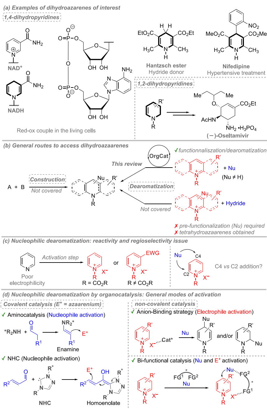
Figure 1. Dearomatization of azaarene: general considerations. * was used to indicate that catalysts are chiral.
