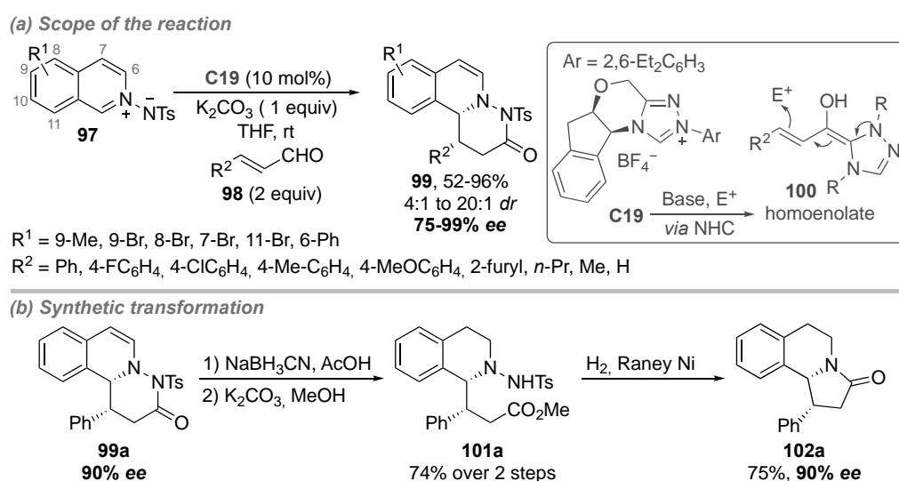
Scheme 31. (3 + 3) cycloaddition to azomethine imines 97 catalyzed by NHC.
