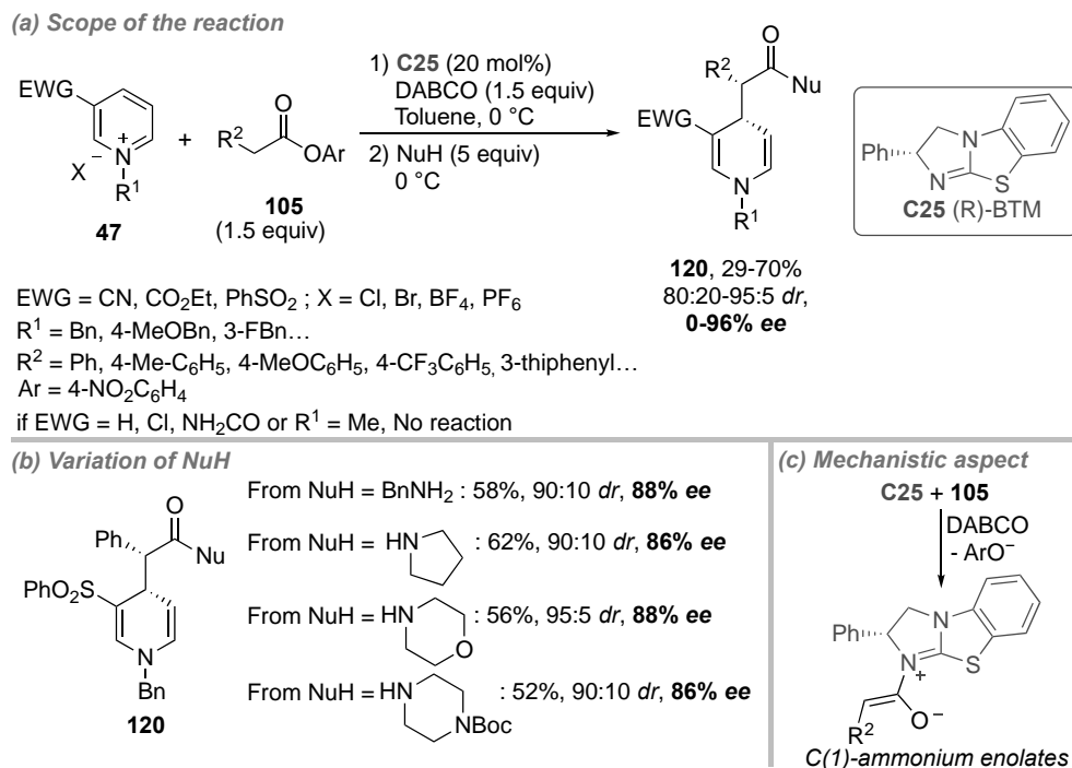
Scheme 37. C4-addition of aryl esters 105 to N -alkyl pyridinium salts 47 catalyzed by NHC.
