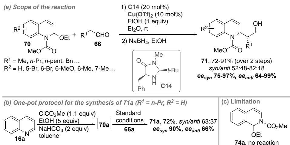
Scheme 21. Diastereo- and enantioselective dearomatization of in situ formed quinolinium salts 70 via synergistic Cu(OTf) 2 /chiral secondary amine catalyst C14 .
