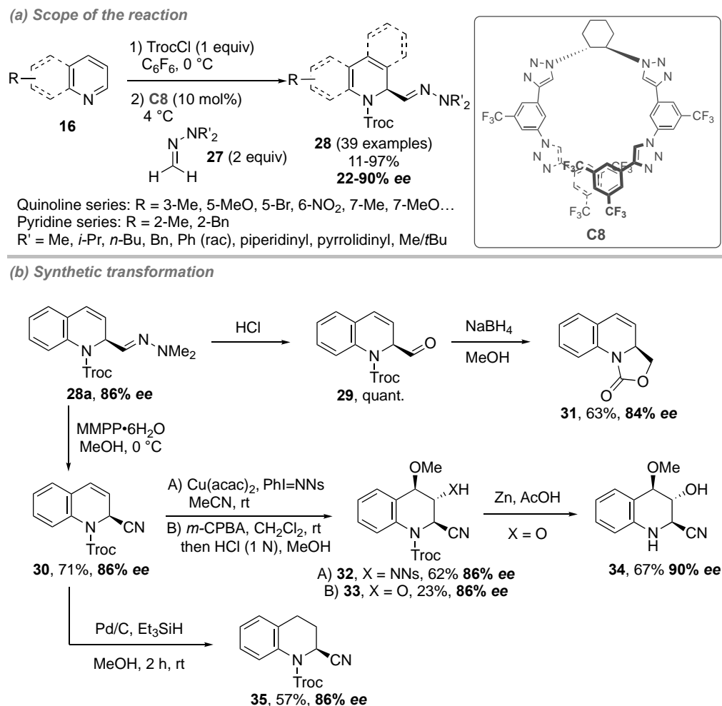
Scheme 11. Addition of N,N-hydrazone 27 to quinolinium salts catalyzed by chiral oligotriazole C8 .
