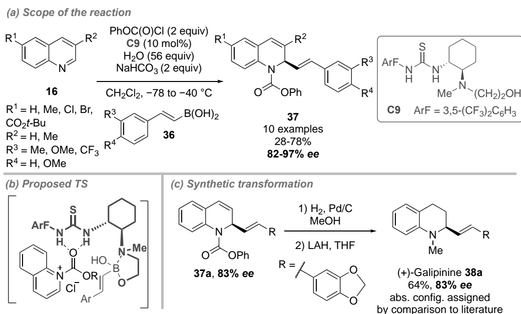
Scheme 12. Addition of boronic acids 36 to quinolinium salts catalyzed by bifunctional catalyst C9 .
