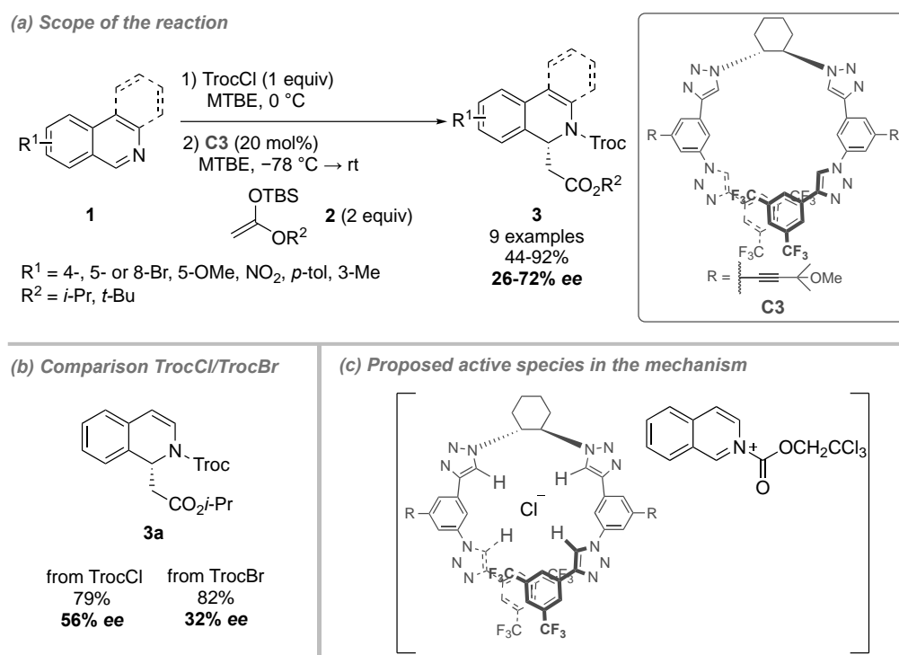
Scheme 3. Reissert-type addition of silyl ketene acetals catalyzed by chiral oligotriazole C3.
