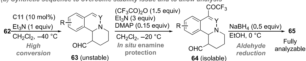
Scheme 18. Diastereo- and enantioselective annulation reaction for the dearomatization of isoquinolinium salts 62 catalyzed by aminocatalyst C11 .
