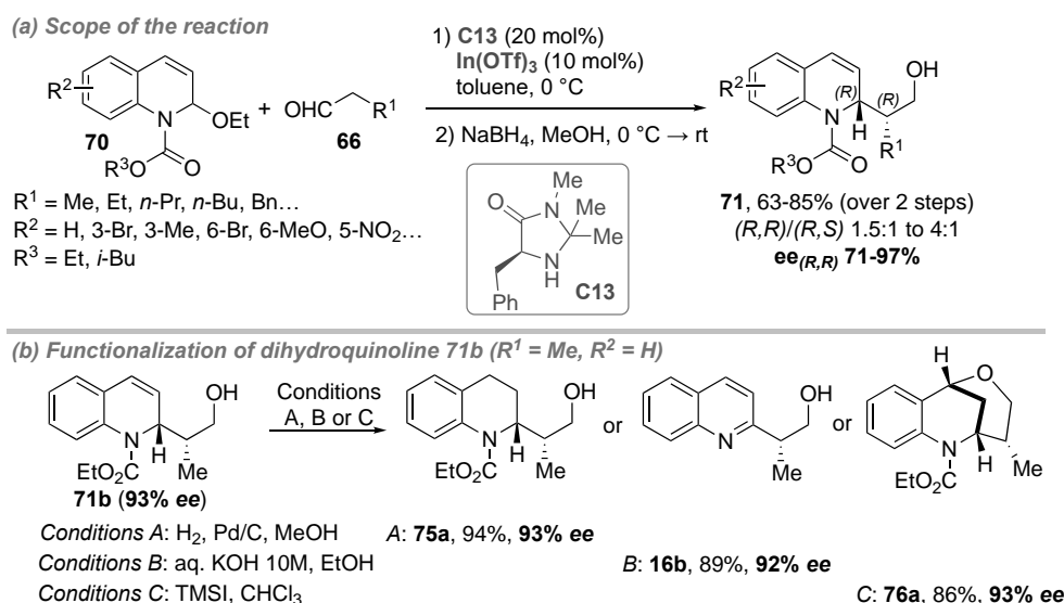
Scheme 22. Diastereo- and enantioselective dearomatization of in situ formed quinolinium salts 70 via synergistic In(OTf) 3 /chiral secondary amine catalyst C13 .
