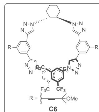
Scheme 13. Addition of ketene silyl acetal 2a to pyridinium salts catalyzed by chiral oligotriazole C6 .
