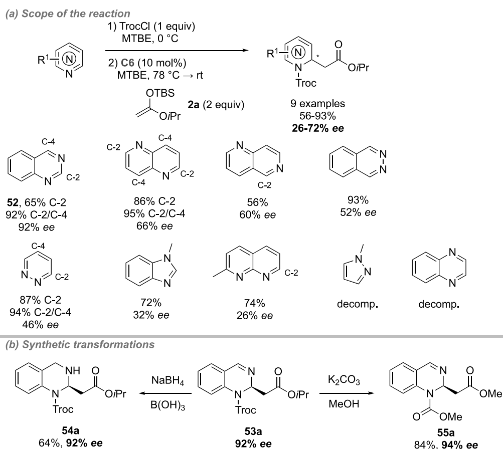
Scheme 16. Addition of silyl ketene acetal 2a to diazaarene salts by chiral oligotriazole C6 .
