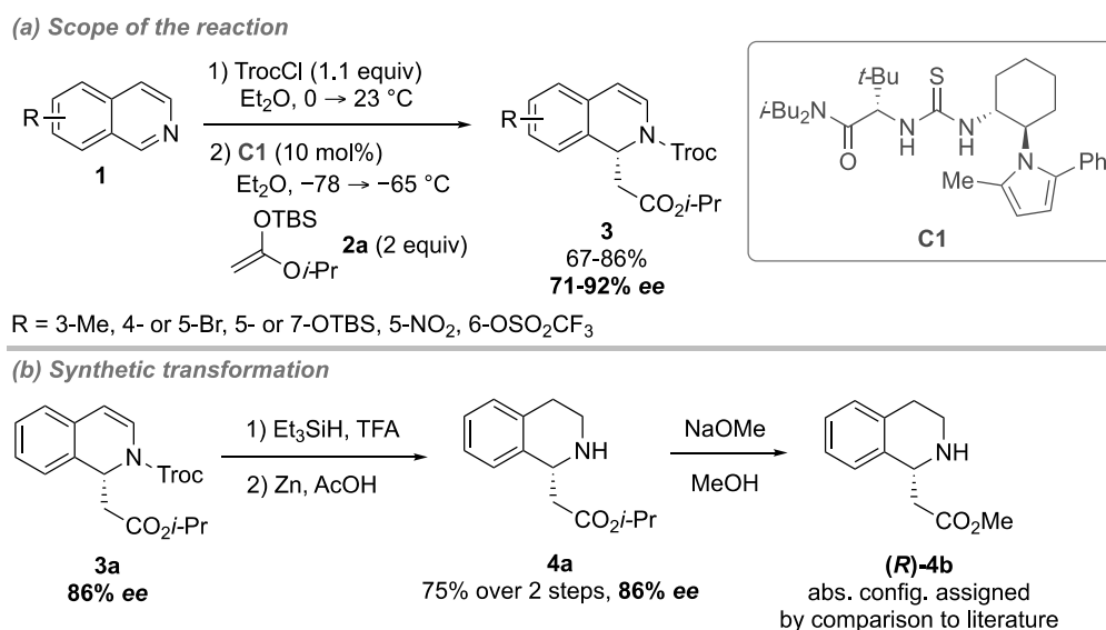
Scheme 1. Reissert-type addition of silyl ketene acetal 2a catalyzed by chiral thiourea C1 .
