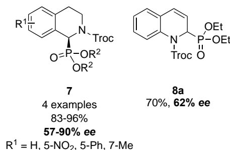
Scheme 4. Addition of silyl phosphites 6 to isoquinolinium salts catalyzed by chiral thiourea C4 .
