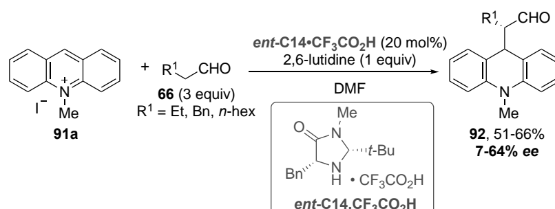
Scheme 28. Asymmetric dearomatization of acridinium salt 91a catalyzed by ent - C14 · \text{CF}_3\text{CO}_2\text{H} .
