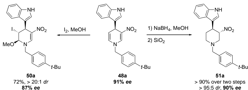
Scheme 15. Addition of indoles to N -alkylpyridinium salts 47 catalyzed by chiral thiourea C10 .
