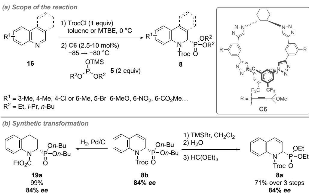
Scheme 8. Addition of silyl phosphites 5 to quinolinium salts catalyzed by chiral oligotriazole C6 .
