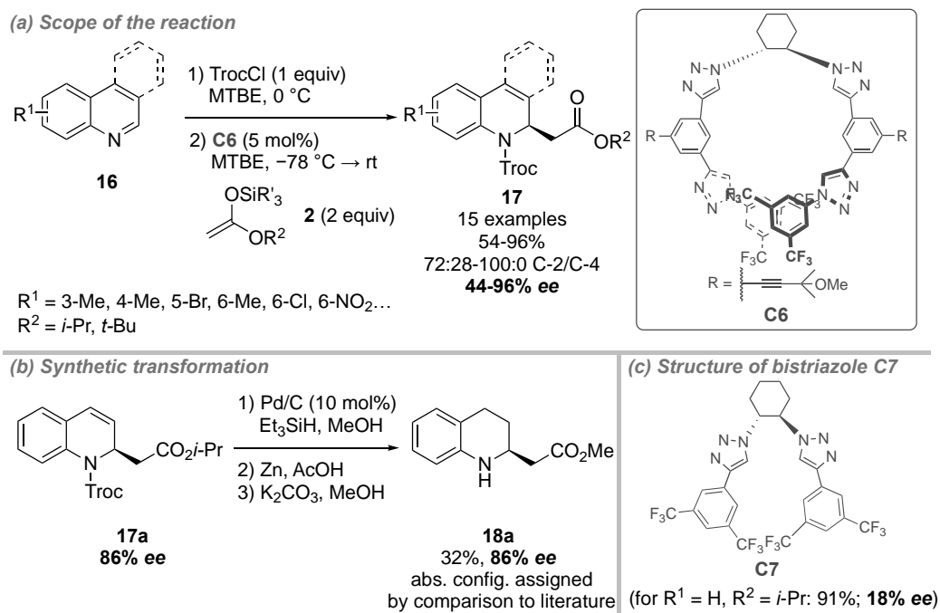
Scheme 7. Addition of ketene silyl acetals 2 to quinolinium salts catalyzed by chiral oligotriazole C6 .
