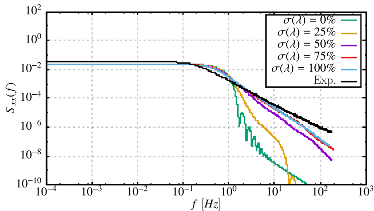
Fig. 15. Influence of \sigma(\lambda) on the spectral representation for a Gaussian kernel ( \lambda = 0.5 and R_f = 2 ) and comparison with experimental data provided by Medina et al. [41] (for I_\infty = 15\% and U_\infty = 0.8 m/s).
