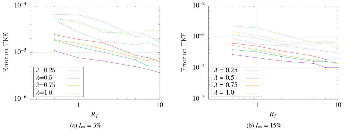
Fig. 9. Average error (full lines) and maximal error (dashed lines) on the value of the TKE K plotted against the filling ratio R_f , for various size of turbulent structures \lambda . For both the cases of low turbulence intensity (a) and high turbulence intensity (b): \sigma(\lambda) = 0\% , and the sub-function f_\lambda uses the Gaussian kernel.
