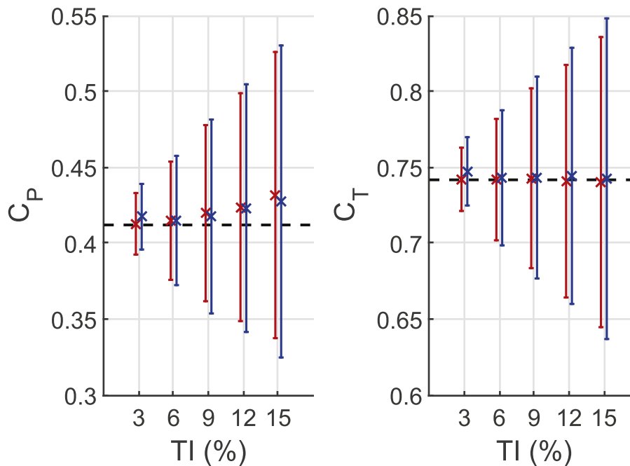
Fig. 5. Power and thrust coefficients for simulations of turbine at optimum TSR of 4.4 under a range of turbulent conditions ( TI = 3, 6, 9, 12, 15\% ). Dashed black lines indicate values of power and thrust coefficient in steady flow conditions; crosses and bars indicate coefficient mean values and standard deviations. Results from SEM turbulence are shown in red and those from Sandia turbulence in blue. Note that SEM results are shown with a slight negative offset in TI and Sandia results with a slight positive offset to make it easier to distinguish the results of the different methods, but the actual TI values are as indicated above. (For interpretation of the references to colour in this figure legend, the reader is referred to the Web version of this article.)
