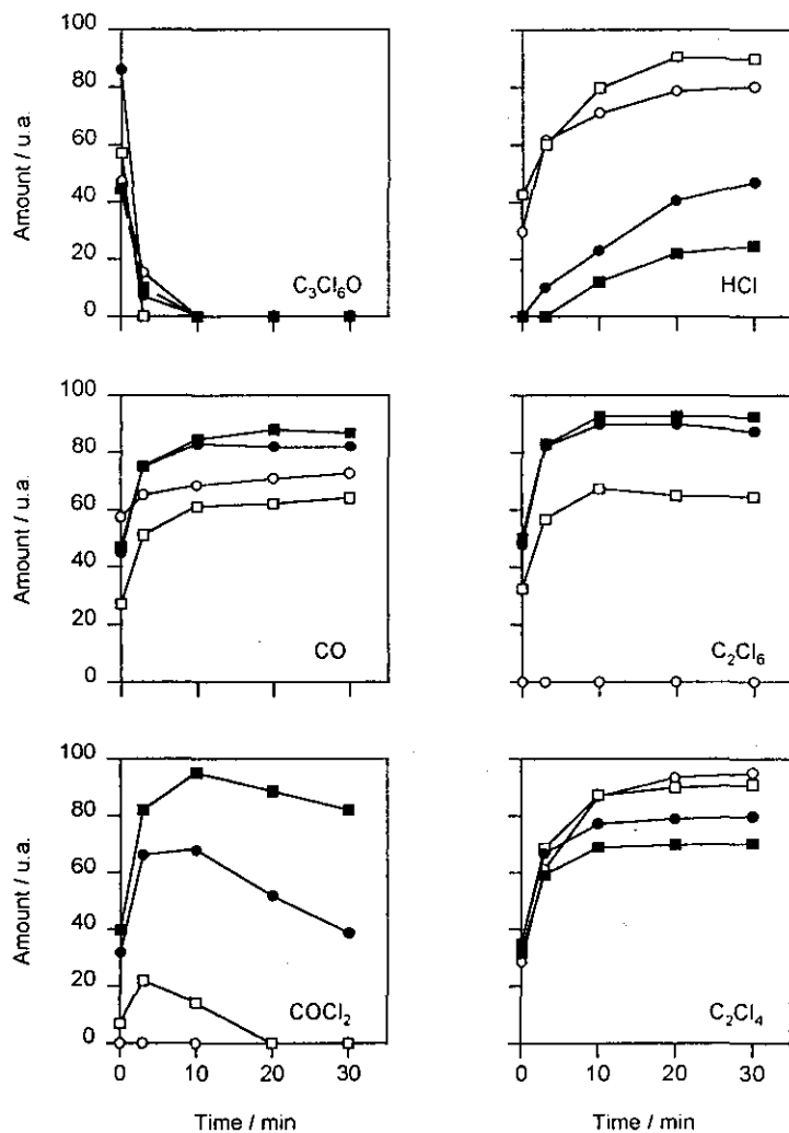
Fig 4. Reaction of C_3Cl_6O with alumina at T = 550 K: variation of the relative amounts (au) of C_3Cl_6O , HCl, CO, C_2Cl_6 , COCl_2 and C_2Cl_4 along: ○ run 1; □ run 3; ● run 6; ■ run 14.
