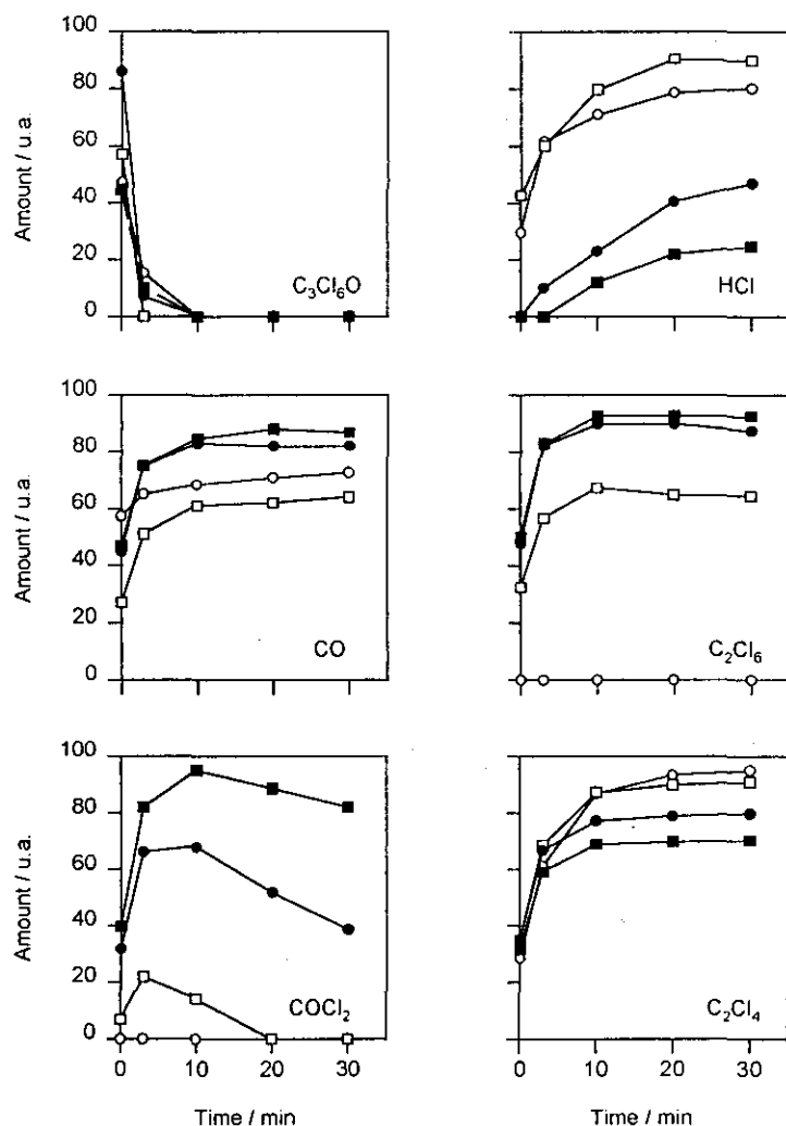
Fig 4. Reaction of \text{C}_3\text{Cl}_6\text{O} with alumina at T = 550\text{ K} : variation of the relative amounts (au) of \text{C}_3\text{Cl}_6\text{O} , \text{HCl} , \text{CO} , \text{C}_2\text{Cl}_6 , \text{COCl}_2 and \text{C}_2\text{Cl}_4 along: \circ run 1; \square run 3; \bullet run 6; \blacksquare run 14.
