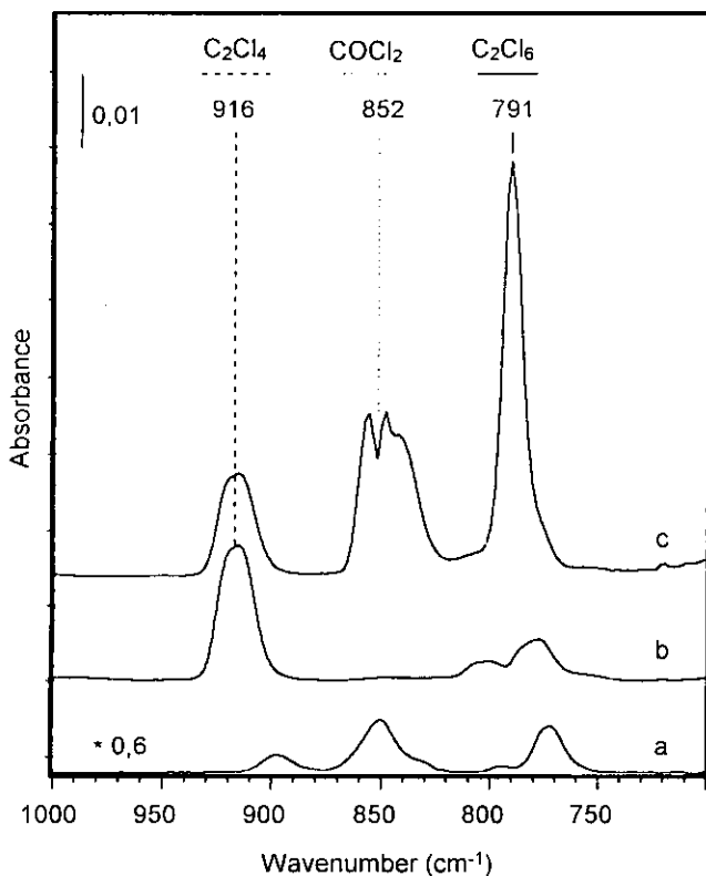
Fig 3. Reaction of \text{C}_3\text{Cl}_6\text{O} with alumina at T = 550 K. Infrared spectra (region 700–1000 \text{cm}^{-1} ) recorded through the gas phase: a) pure \text{C}_3\text{Cl}_6\text{O} ; b) after 10 min contact with the first dose of \text{C}_3\text{Cl}_6\text{O} ; c) after 10 min contact with the tenth dose of \text{C}_3\text{Cl}_6\text{O} .
