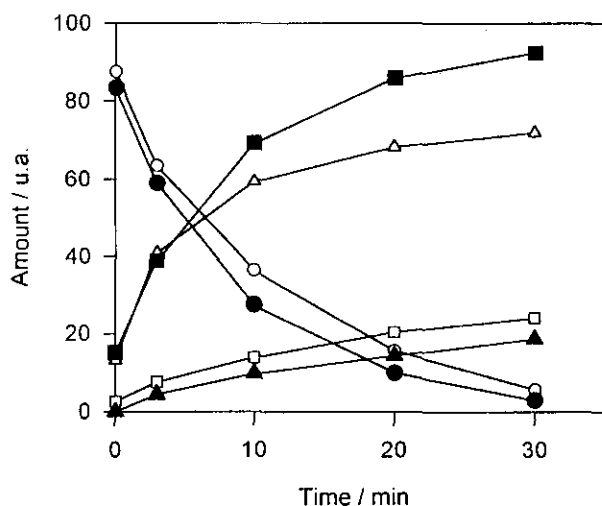
Fig 2. Reaction of \text{C}_2\text{Cl}_6 with alumina at T = 650 K: variation of the relative amounts (ua) of compounds with time. Run 1: \text{C}_2\text{Cl}_6 ●; \text{C}_2\text{Cl}_4 ▲; HCl ■. Run 9: \text{C}_2\text{Cl}_6 ○; \text{C}_2\text{Cl}_4 △; HCl □.
