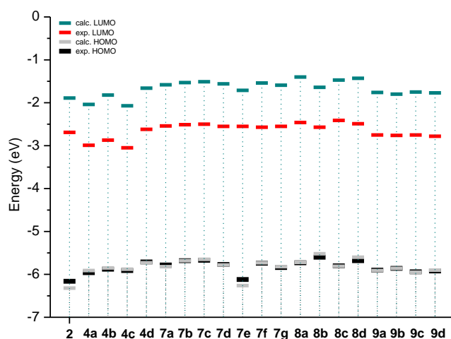
Figure 8. Compilation of empirical and theoretical obtained HOMO-LUMO energy levels. Calculation level DFT TDDFT/B3LYP in \text{CH}_2\text{Cl}_2 .
