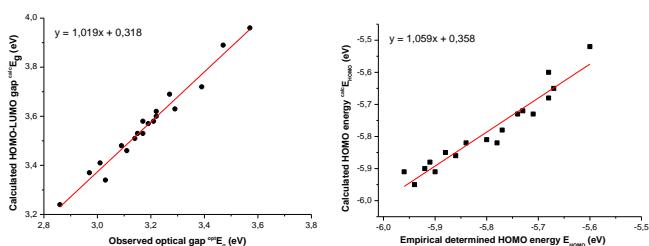
Figure 9. (left) Correlation between observed and calculated band gaps ( E_g ). (right) Correlation between HOMO energy levels obtained by electrochemical methods ( E_{\text{HOMO}} ) and calculated HOMO energies ( ^{calc}E_{\text{HOMO}} ). Calculation level DFT TDDFT/B3LYP for both.
