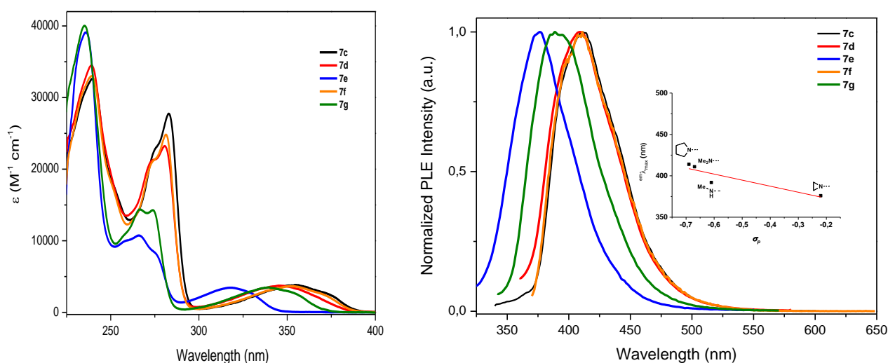
Figure 4. Comparative absorption (left) and photoluminescence emission spectra (right) of representative 2- N -amino-4-methoxyquinazolines with varying N -amino substituents recorded in \text{CH}_2\text{Cl}_2 ( c = 10^{-5} M). Inset: Correlation of the Hammett substitution parameter \sigma_{\text{p}} with the wavelength \text{em}\lambda_{\text{max}} of the PLE intensity maxima.
