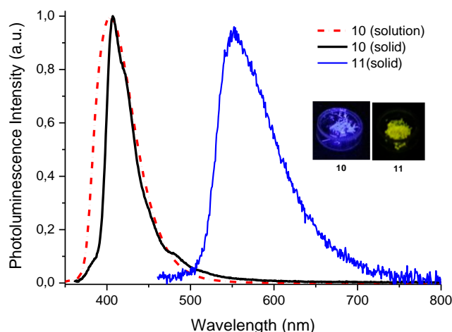
Figure 6. PLE spectra of 2- N -morpholino-4,6,7-trimethoxyquinazoline (10) in solution and from solid state; and solid state PLE spectra of 2- N -morpholino-6-nitro-4-methoxyquinazoline (11). Compound 11 is non-fluorescent in solution. Insert: Quinazoline 10 and 11 (solid) under UV-lamp.
