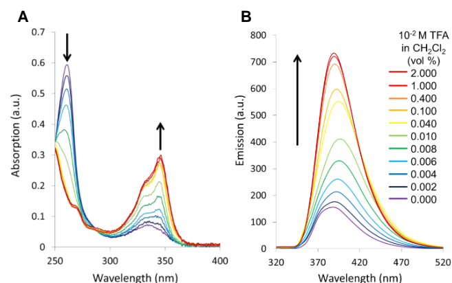
Figure 10. A) Successive changes of UV-vis absorption bands of 7-amino-2-morpholino-4-methoxyquinazoline ( 12 ) on addition of aliquots of trifluoroacetic acid (TFA). B) Fluorescence emission intensity enhancement of quinazoline 12 on ratiometric titration with TFA.
