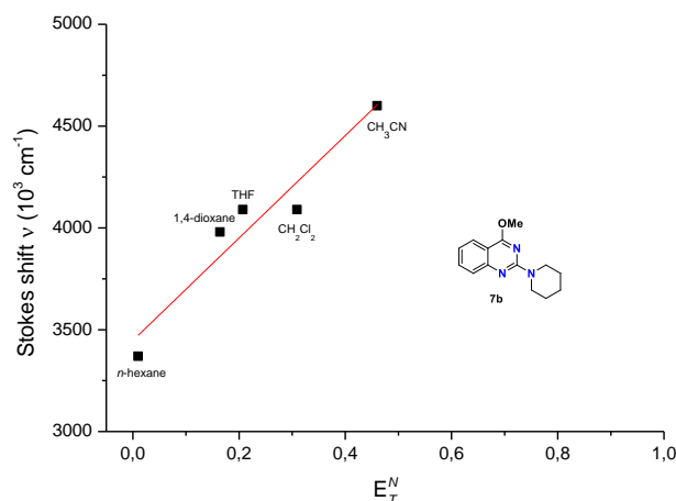
Figure 5. Solvatochromism of 2- N -piperidino-4-methoxyquinazoline (7b). Correlation of Reichardt's normalized polarity parameter E_T^N with obtained Stokes shift. E_T^N values: 0.01 ( n -hexane), 0.164 (1,4-dioxane), 0.207 (THF), 0.309( \text{CH}_2\text{Cl}_2 ), and 0.460 ( \text{CH}_3\text{CN} ).
