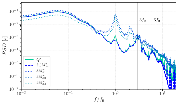
Fig. 25. Comparison of the power spectral densities of the rotor torque and the edgewise blade root bending moments obtained for the ATIR turbine for TSR = 4.7, U_\infty = 1.2 m/s and the HTI case.
