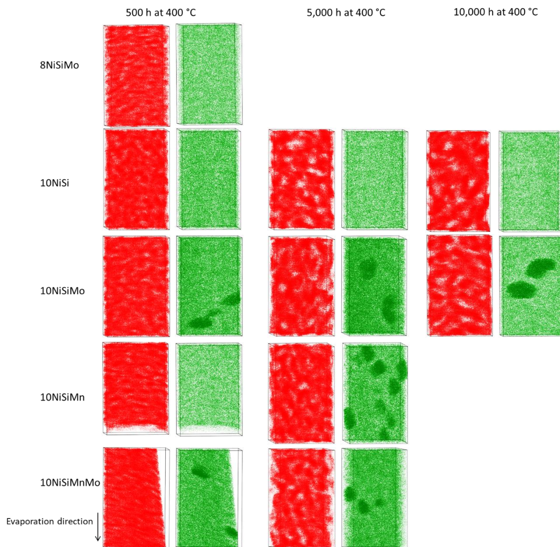
Figure 4: Distribution of Cr atoms (in red) and Ni + Si + Mo + Mn atoms (in green) after ageing of 500 h, 5,000 h and 10,000 h at 400 °C for 8NiSiMo, 10NiSi, 10NiSiMo, 10NiSiMn and 10NiSiMnMo. Volume=30x30x50 nm 3 . V=30x30x43 nm 3 . (Color online)
