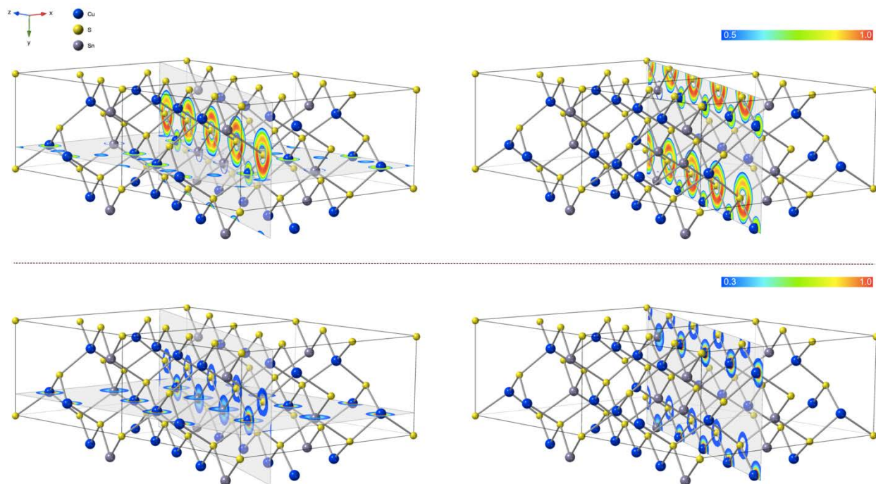
Figure 12. Contour of the Electron Localization Factor (ELF) (top) and charge density (bottom) for selected planes of monoclinic C2 Cu_5Sn_2S_7 . Values for the ELF range between 0 and 1: ELF = 0.5 (blue contours) indicates free electron behavior and ELF = 1.0 (red contour) indicates perfect
