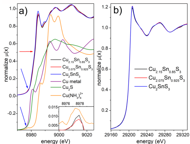
Figure 8. XANES spectra: a) Cu K-edge and b) Sn K-edge, for \text{Cu}_2\text{SnS}_3 (blue curve), \text{Cu}_{2.075}\text{Sn}_{0.925}\text{S}_3 (red curve) and \text{Cu}_{2.15}\text{Sn}_{0.85}\text{S}_3 (black curve). The inset in a) focuses on a region around the quadrupolar 1s \rightarrow 3d transition peak. In order to isolate such transition from the background, the spectrum of \text{Cu}_2\text{SnS}_3 have been subtracted from \text{Cu}_{2.15}\text{Sn}_{0.85}\text{S}_3 (black curve) and
