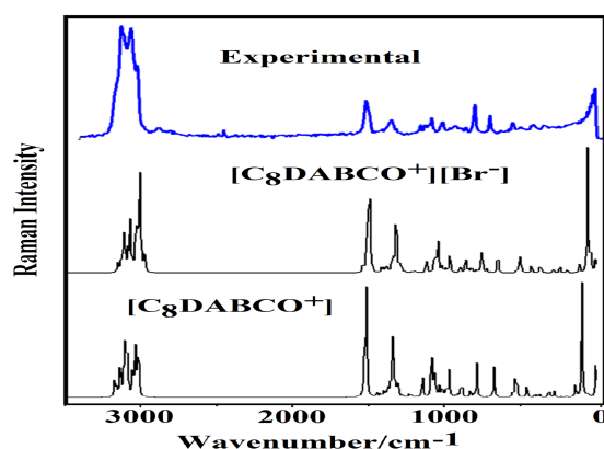
Figure 7. Experimental FT-Raman of [\text{C}_8\text{DABCO}^+][\text{Br}^-] ionic liquid in the solid phase compared with the corresponding predicted for IL and cation in gas phase by using the hybrid B3LYP/6-31G* method.
