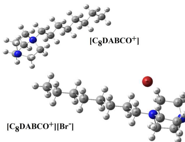
Figure 3. Optimized theoretical structures of [\text{C}_8\text{DABCO}^+][\text{Br}^-] IL and its cation by using the hybrid B3LYP/6-31G* method together with atoms labeling.
