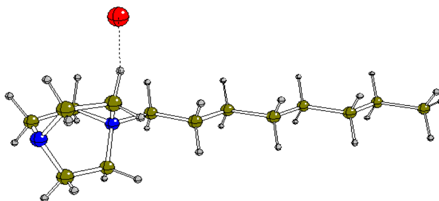
Figure 4. Monodentate coordination proposed between cation and anion of [C 8 DABCO + ][Br - ] ionic liquid in gas phase by using the B3LYP/6-31G* method showing the formation of strongest C6-H6...Br46 interaction.
