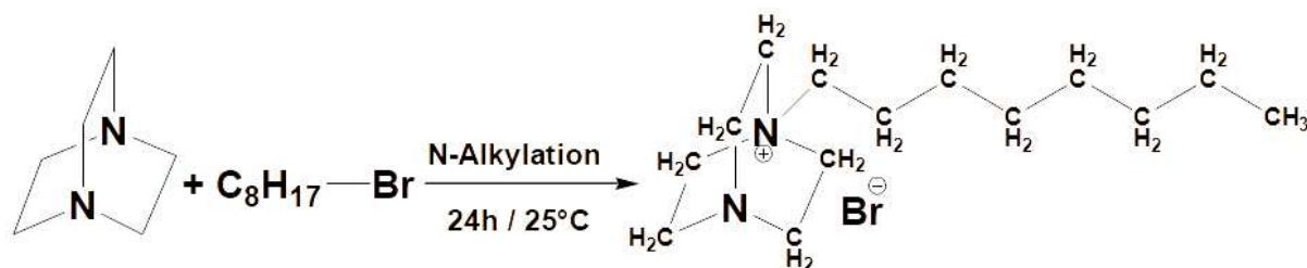
Scheme 1. General synthesis of [\text{C}_8\text{DABCO}^+][\text{Br}^-] .
