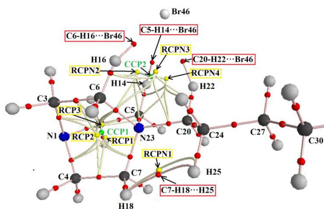
Figure 5. Molecular graphic of [\text{C}_8\text{DABCO}^+][\text{Br}^-] ionic liquid in gas phase by using the B3LYP/6-31G* method showing the BCP and the RCPs and the CCPs.
