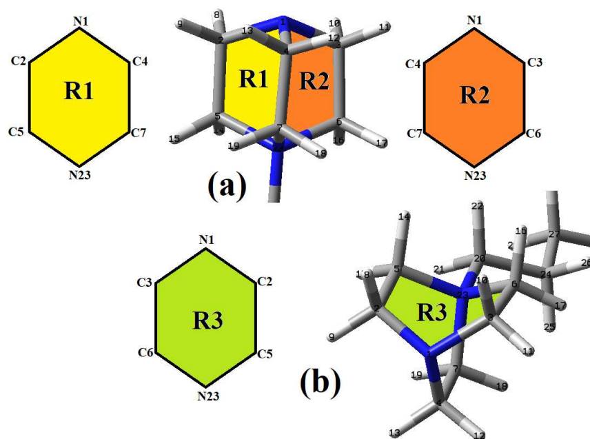
Figure 1. Two different positions of cage corresponding to the molecular structure of [C_8DABCO^+] cation with the identifications of two R1 and R2 rings (a) and R3 ring (b) with the labeling of involved atoms. To a better observation the side chain was not considered.
