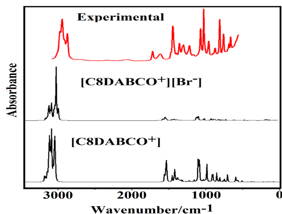
Figure 6. Experimental FT-IR of [\text{C}_8\text{DABCO}^+][\text{Br}^-] ionic liquid in the solid phase compared with the corresponding predicted for IL and cation in gas phase by using the hybrid B3LYP/6-31G* method.
