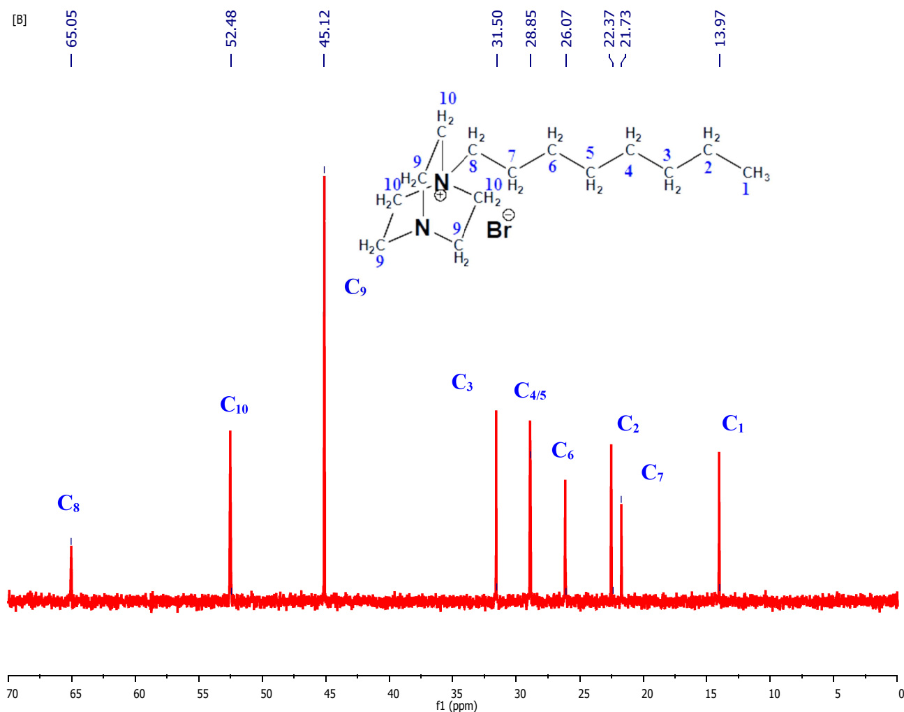
Figure 2. Hydrogen atom labeling and ^1H NMR (a), carbon atom labeling and ^{13}C NMR (b) in CDCl_3 , of [C_8DABCO^+][Br^-] .
