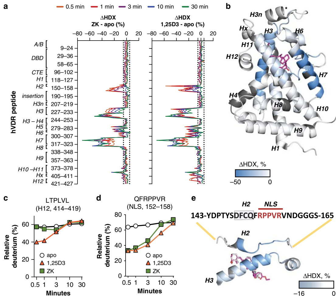
Fig. 2 Ligand-induced hVDR conformational changes. a Differential deuterium uptake ( \Delta HDX) of hVDR between apo and ZK-bound (left panel) or 1,25D3-bound (right panel) hVDR/hRXR \alpha \Delta NTD heterodimers. The VDR LBD is composed of H1–H12. Negative values indicate decreased deuterium incorporation upon ligand binding. Dashed lines represent a \Delta HDX of 5%. b Average \Delta HDX of hVDR between ZK-bound and apo-hVDR/hRXR \alpha \Delta NTD heterodimers across the various time points mapped onto hVDR LBD (PDB: 1DB1 44 ). Regions not covered by HDX-MS are shown in dark gray. Differential deuterium uptake plots of the hVDR residues 414–LTPLVL–419 located in H12 ( c ) and of 152–QFRPPVR–158 located in the H1–H3 loop ( d ) determined in ZK-bound, 1,25D3-bound and apo hVDR/hRXR \alpha \Delta NTD heterodimers. e Zoom of average \Delta HDX across the various time points of the VDR region encompassing H2 and a nuclear localization signal (NLS) mapped onto the hVDR LBD (PDB: 1DB1 44 ). HDX-MS data were collected in triplicates, and deuteration data were normalized to the maximal theoretical uptake ( \pm s.e.m.).
