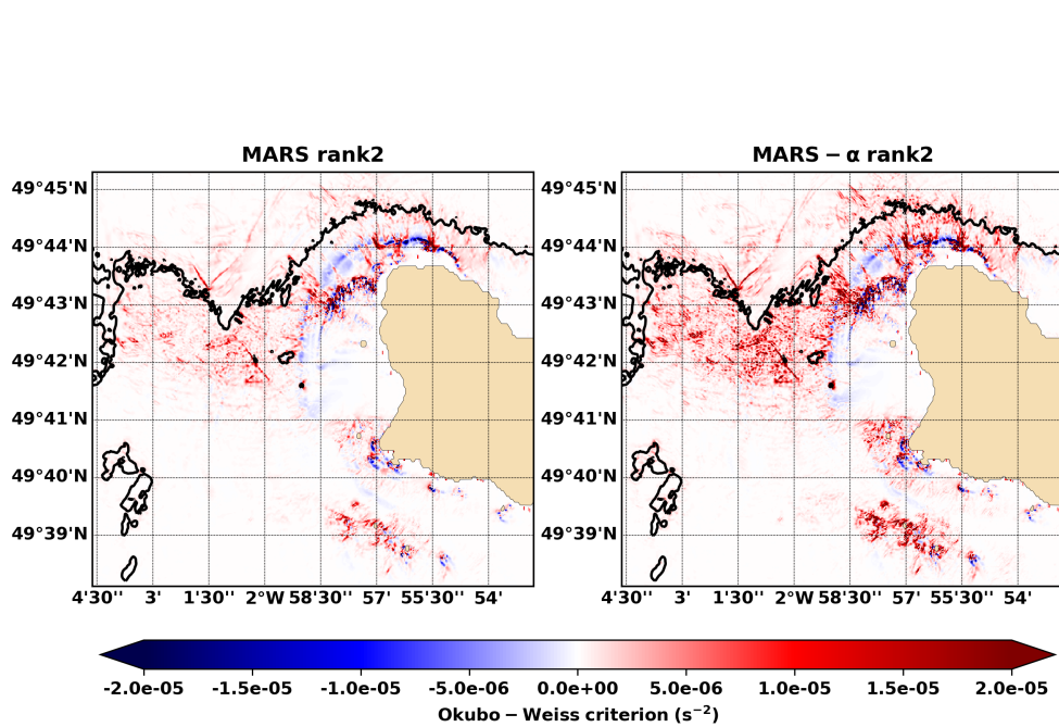
Fig. 8. Okubo-Weiss criterion computed with barotropic currents for the ebb maximum currents period: MARS Rank2 (left panel) and MARS- \alpha Rank2 (right panel) with a constant vertical viscosity. Bathymetric contours are shown with a grey scale, ranging from 20 meters (white) to 40 meters (black).
