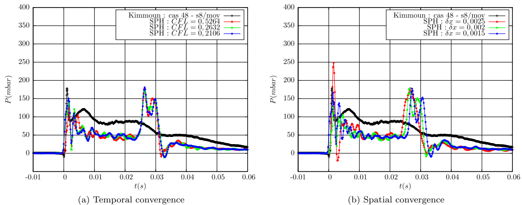
Figure 18. Time evolution of the pressure. Altitudes of the sensors in the experiences of Kimmoun et al. [57] is 0.073 m above the beach. t = t_{\text{sim}} - 8.88 s. Simulation parameters : h = 0.713 m, a = 0.0864 m (cf. Table 3). The numerical pressure records were obtained by applying a moving average over 5 \delta t .
