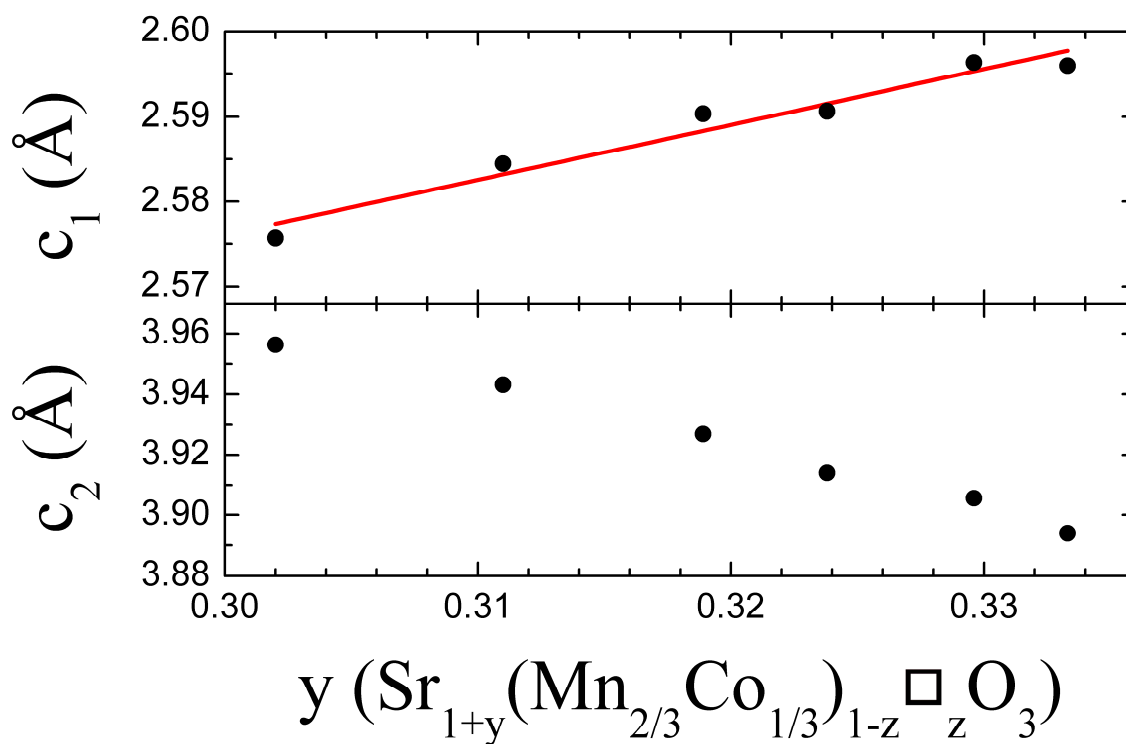
Fig.8 Evolution of the cell parameters of the oxides \text{Sr}_{1+y}[(\text{Mn}_{2/3}\text{Co}_{1/3})_{1-z}\square_z]\text{O}_3 versus y
