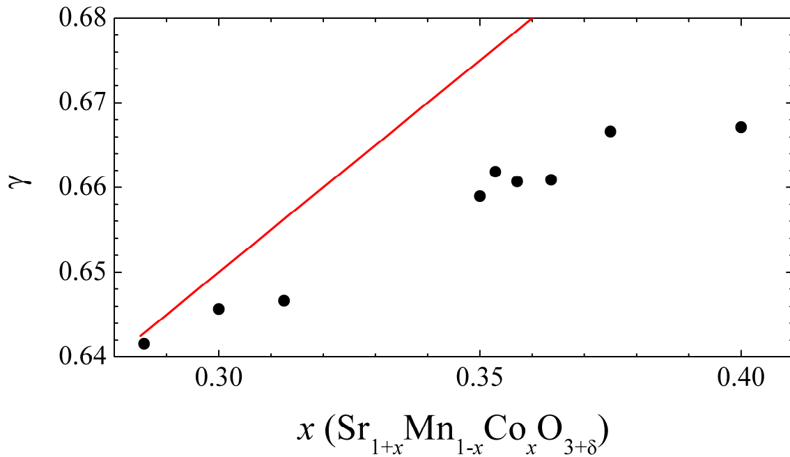
Fig.4 Evolution of the modulation vector \gamma versus the cobalt content x of the oxides \text{Sr}_{1+x}(\text{Mn}_{1-x}\text{Co}_x)\text{O}_{3+\delta} . The red line is the relationship between the composition x and the modulation vector \gamma_x expected for this composition: \gamma_x = (x+1)/2 .
