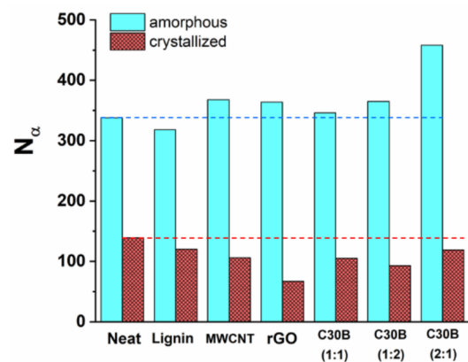
Figure 5. Number of relaxing units per CRR in amorphous and semi-crystalline PLLA and nanocomposites. Dashed lines are a guide, showing N_g for amorphous neat PLLA.
