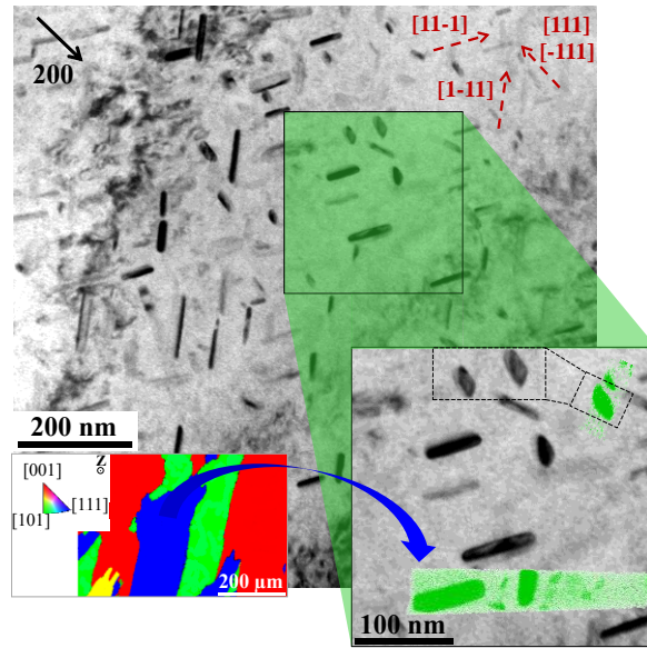
Figure 4: TEM image of the low dose rate irradiated Fe3%Ni alloy, taken in a (011) zone axis along g=[200] , presenting elongated precipitates and scaled APT reconstructed volumes showing Ni-rich clusters (on the top and the bottom of the magnified image). The EBSD map recorded before the extraction of the tip presented is also given at the bottom-left.
