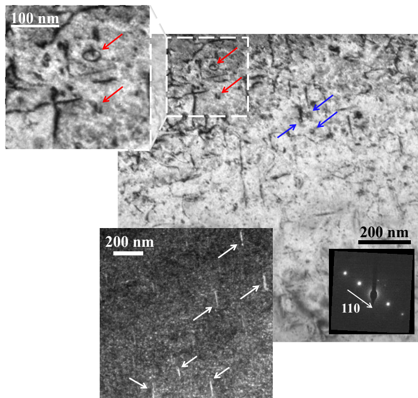
Figure 7: TEM images of the Fe3%Mn sample irradiated at low dose rate, taken in a \{001\} zone axis, along g = \langle 110 \rangle , in BF mode. A magnified image is presented on the upper-left corner to highlight the presence of small \frac{1}{2} \langle 111 \rangle dislocation loops, in addition to large \langle 100 \rangle ones appearing edge-on (on the WBDF image, presented on the lower-left corner).
