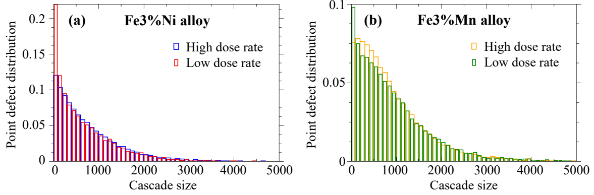
Figure 2: Proportion of each cascade size according to its number of point defects, in (a) the Fe3%Ni alloy, where the results for the high and low dose rates conditions are shown is blue and red respectively; and (b) the Fe3%Mn alloy, where the results for the high and low dose rates conditions are shown is orange and green respectively. Results were obtained using the IRADINA code 52,53 .
