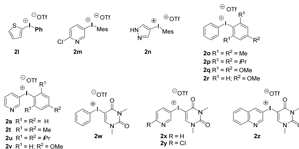
Figure 1. Unsymmetrical diaryliodonium triflates 2l–z that were used in this study.
