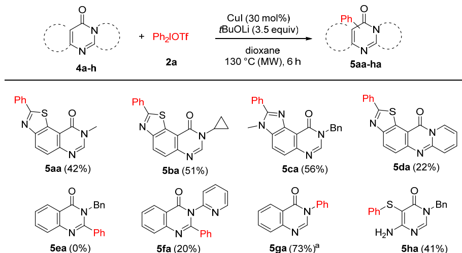
Scheme 3. Scope of fused-pyrimidinone derivatives for the copper-catalyzed C–H arylation. a 3 equiv of 2a was used.
