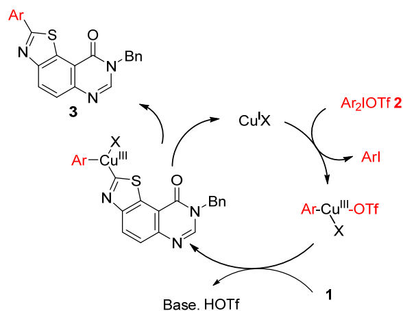
Scheme 4. Plausible mechanism of the copper-catalyzed C–H arylation of heteroarenes with diaryliodonium triflate as arylating reagent.
