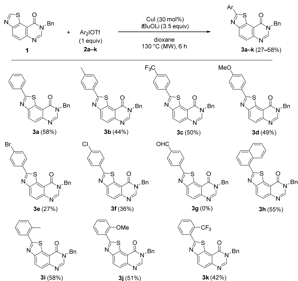
Scheme 2. Scope of diverse diaryliodonium triflates in the copper-catalyzed C–H arylation of N 8 -benzylthiazolo[5,4- f ]quinazolin-9(8 H )-one 1 .
