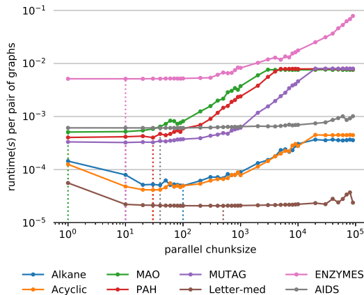
Fig. 3. Runtimes to compute the Gram matrices of the shortest path kernel on each dataset on 28 CPU cores with different chunksize values.
