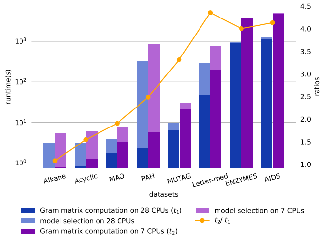
Fig. 2. Left y-axis: Runtimes (in seconds) to compute Gram matrices (bottom of each pillar) and perform model selections (top of each pillar) for the shortest path kernel on each dataset on 28 CPU cores (blue pillar) and 7 CPU cores (magenta pillar) with parallelization. Right y-axis: The orange dots are the ratios between the runtimes to compute Gram matrices of each dataset on 28 and 7 cores.
