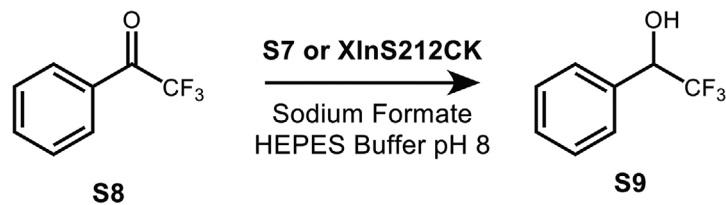
FIG. 4 Hydrogenation of TFAC S8 by sodium formate catalyzed by Knölker's complex S7 or by the XlnS212CK biohybrid.
