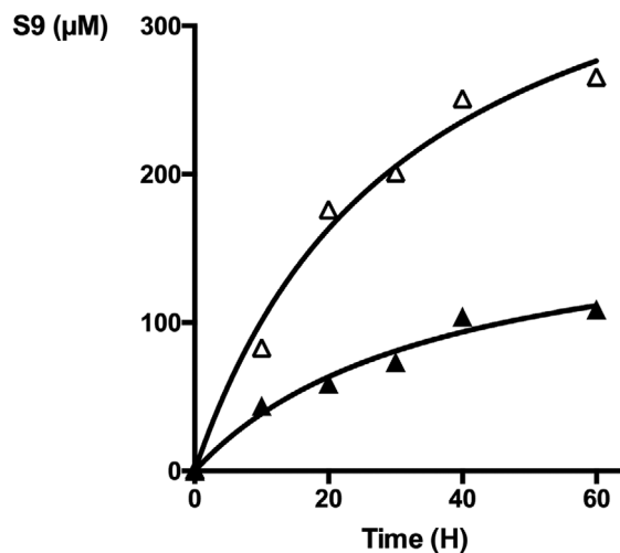
FIG. 5 Time course of hydrogenation of TFAC by XlnS212CK ( \Delta ) in aqueous buffer in comparison with CK alone in EtOH ( \blacktriangle ).
