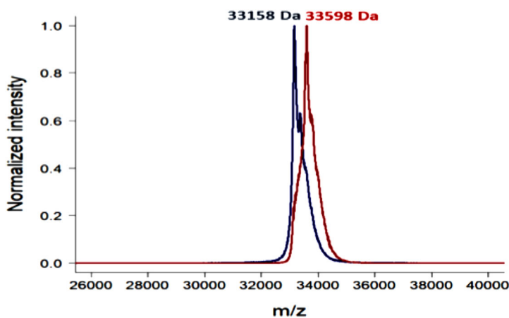
FIG. 3 Maldi-ToF spectra of the XlnS212C variant measured before (blue) and after (red) functionalization with the Knölker's complex compound.
