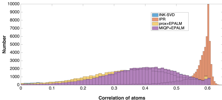
Figure 3: The distribution of the coherence between each two atoms of the proposed algorithms and its comparison to the INK-SVD and IPR algorithms
