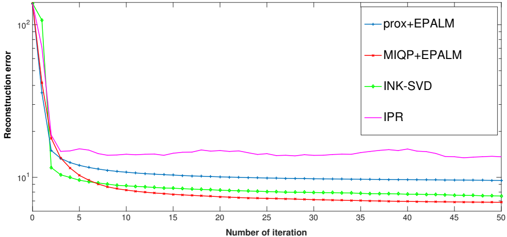
Figure 2: The convergence of the proposed algorithm and its comparison to the INK-SVD and IPR algorithms
