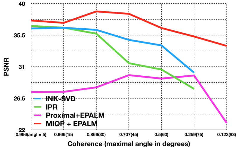
Figure 4: The figure of reconstruction results
