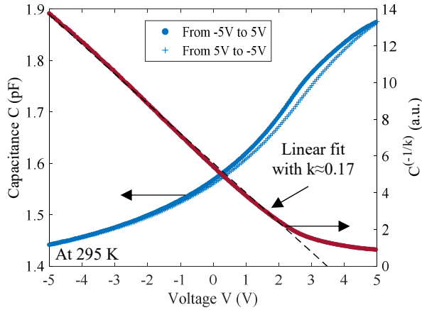
Figure 4. C-V characteristics at room temperature of the GaN p^+n diode showing a hysteresis for voltage between -5 V to 5 V (left y-axis) and the C^{-1/k} -V curve with a linear fit allowing to extract the diffusion barrier of about 3.6 V (right y-axis).
