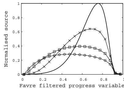
Fig. 7 Thick-line: \omega^+(\tilde{c}) vs \tilde{c} as obtained from a 1D laminar flame (tabulated chemistry). \langle \overline{\omega^+} | \tilde{c} \rangle from DNS vs \tilde{c} for filter sizes \times : 0.3 mm, \square : 0.6 mm, \circ : 0.9 mm, ( \delta_L = 0.4 mm). Reprinted with permission [39].
