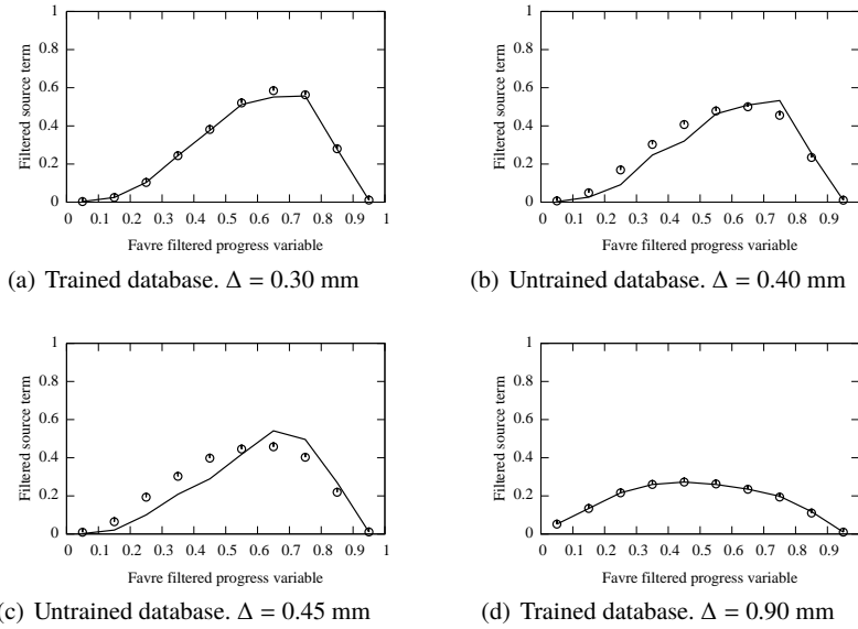
Fig. 12 \langle \bar{\omega}^+ | \bar{c} \rangle vs \bar{c} . Symbols: DNS reference. Line: CNN prediction.
