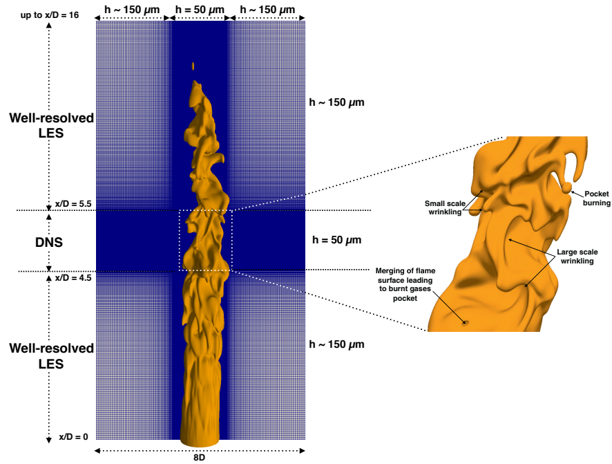
Fig. 6 LES-DNS snapshot of the jet-flame simulation [26]. Mesh and iso-progress variable c = 0.8 . h : resolution. Right: zoom of iso- c = 0.8 in the DNS zone (different angle view). Reprinted with permission [26].
