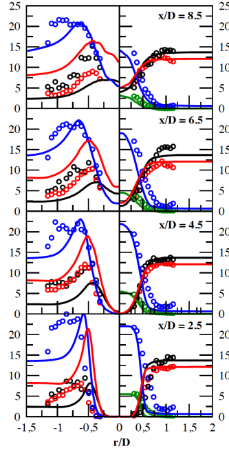
Fig. 3 Mass fractions in %. Symbol measurements [17]. Line: LES. In each subfigure: Left: Red: \text{CO} \times 10 . Black: \text{H}_2 \times 100 . Blue: \text{OH} \times 75 . Right: Blue: \text{O}_2 . Green: \text{CH}_4 . Red: \text{H}_2\text{O} . Black: \text{CO}_2 . Reprinted with permission [26].
