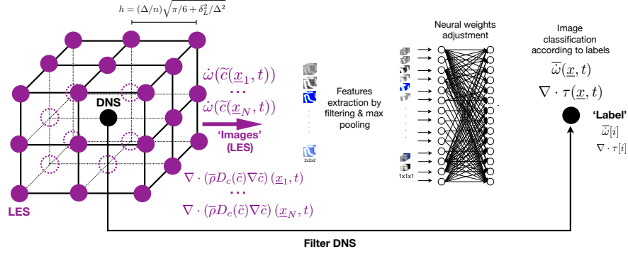
Fig. 9 CNN training from DNS, sketch of the database construction. Reprinted with permission [39].
