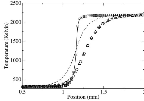
Fig. 1 Temperature profiles across a one-dimensional premixed flame. Line: T(x) ; Square: T^*(x) from deconvolution (Eq. (10)); Dash: \bar{T}(x) ; Circle: \tilde{T}(x) . Solving balance equation for filtered 1D flame from deconvolution Triangle: \tilde{T}(x) . \Delta/\delta_{fl} = 8 . Reprinted with permission [13].
