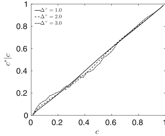
Fig. 4 Conditionally averaged progress variable as obtained from IDEF based on the actual value as obtained from the DNS. \Delta^+ = \Delta/\delta_L Reprinted with permission [11].
