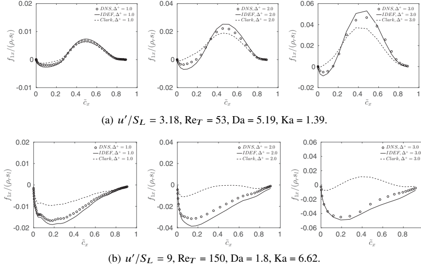
Fig. 5 SGS convective flux in the direction normal to the mean flame front averaged in the transverse plane, plotted versus a progress variable ( c_x = 0 in fresh gases and c_x = 1 in fully burnt gases). \circ : DNS. —: IDEF. ---: Clark model [32]. Left: \Delta/\delta_L = 1 , Middle: 2, Right: 3. Reprinted with permission [31].
