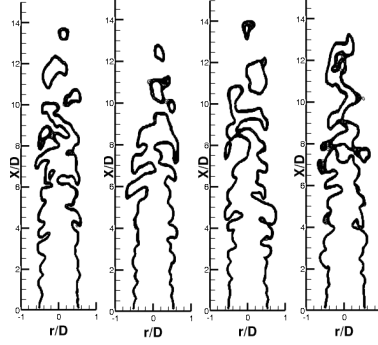
Fig. 2 Time sequence of iso-filtered source of progress variable, \Delta t = 1.8 ms. Reprinted with permission [13].
