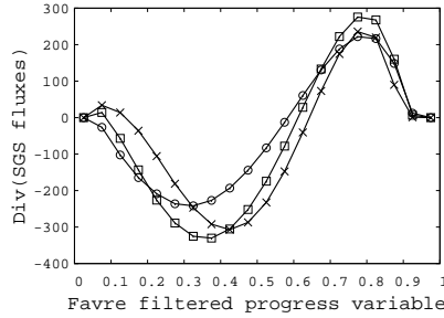
Fig. 8 \langle \nabla \cdot \tau | \tilde{c} \rangle vs \tilde{c} . Filter size \times : 0.3 mm, \square : 0.6 mm, \circ : 0.9 mm. Reprinted with permission [39].
