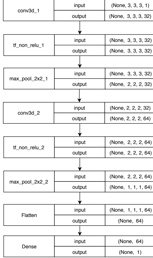
Fig. 10 Typical structure of a convolutional network for scalar deconvolution. More details on the TensorFlow functions used may be found in [39]. Reprinted with permission [39].
