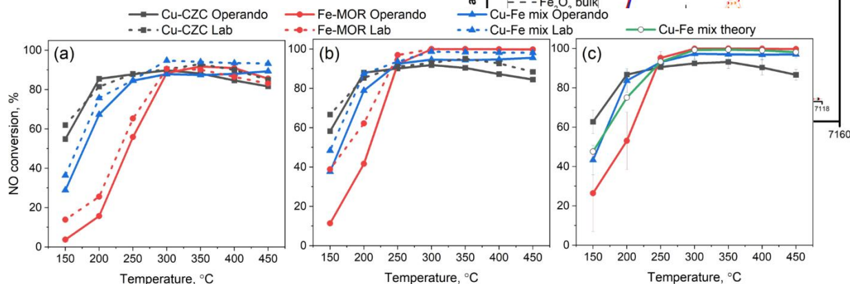
Figure 1 (a) NO conversion measured for Cu-CZC, Fe-MOR and their mechanical mixture during operando XAS experiment and in the lab with similar mass of the catalyst pellets and total flux. (b) NO conversion data recalculated for relevant reaction conditions (GHSV = 50 000 h -1 ) as detailed in Section 1 of SI (c) Experimental NO conversion curves recalculated using the kinetic constants averaged over operando XAS and laboratory experiments together with the theoretical curve (green curve) simulated for the mixed material for the case when its Cu-CZC and Fe-MOR components work independently
