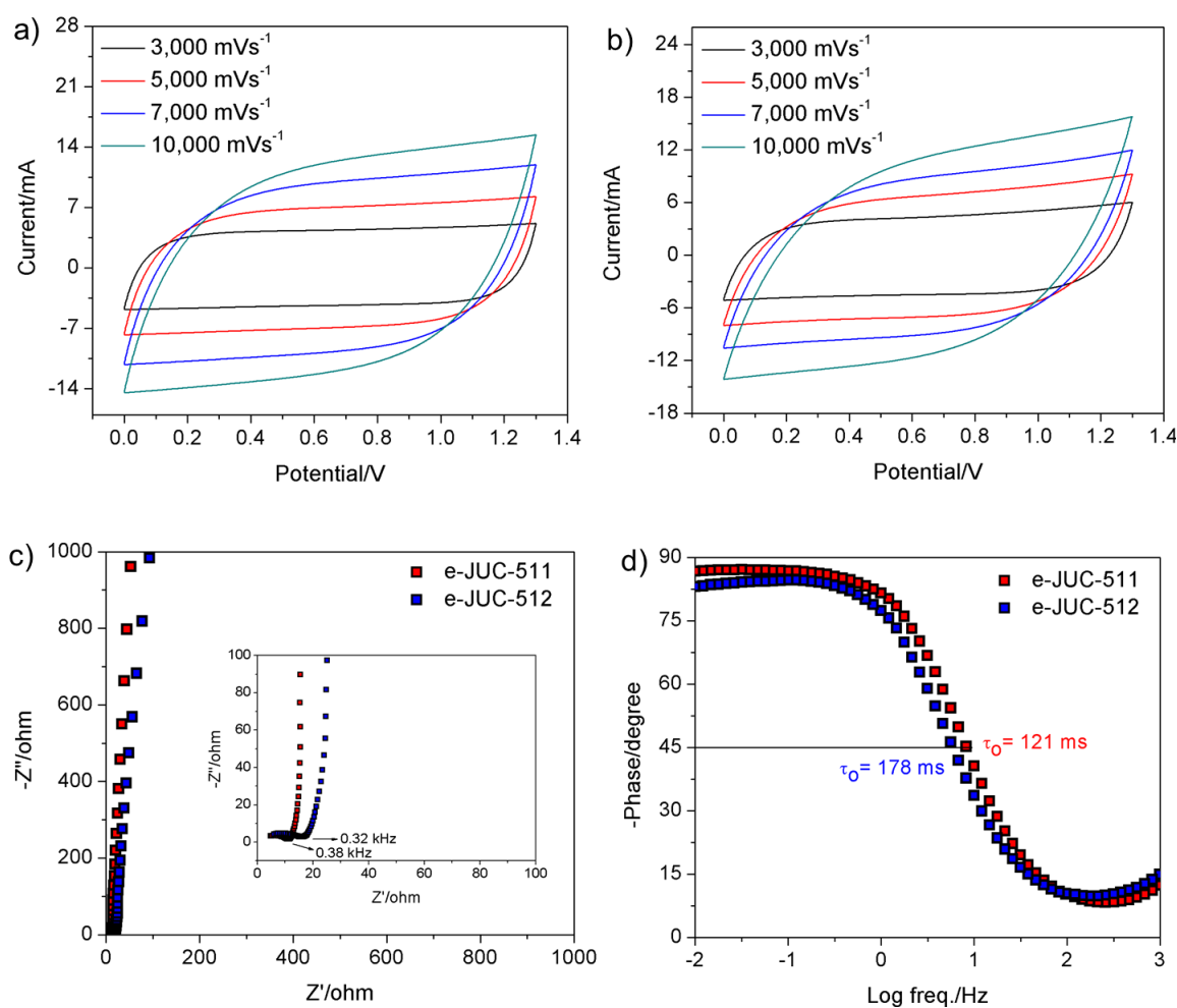
Figure 4. Capacitive performances of e-COF capacitor cells: a) CV curves of e-JUC-511 capacitor cell at scan rate 3,000–10,000 mV s -1 with preservation of rectangular shape. b) CV curves of e-JUC-512 capacitor cell at scan rate 3,000–10,000 mV s -1 with preservation of rectangular shape. c) Nyquist plot of e-JUC-511 and e-JUC-512 capacitor cells at frequency range 10 mHz–100 kHz and amplitude of 10 mV. d) Bode plot of e-JUC-511 and e-JUC-512 capacitor cells with low \tau_0 values.
