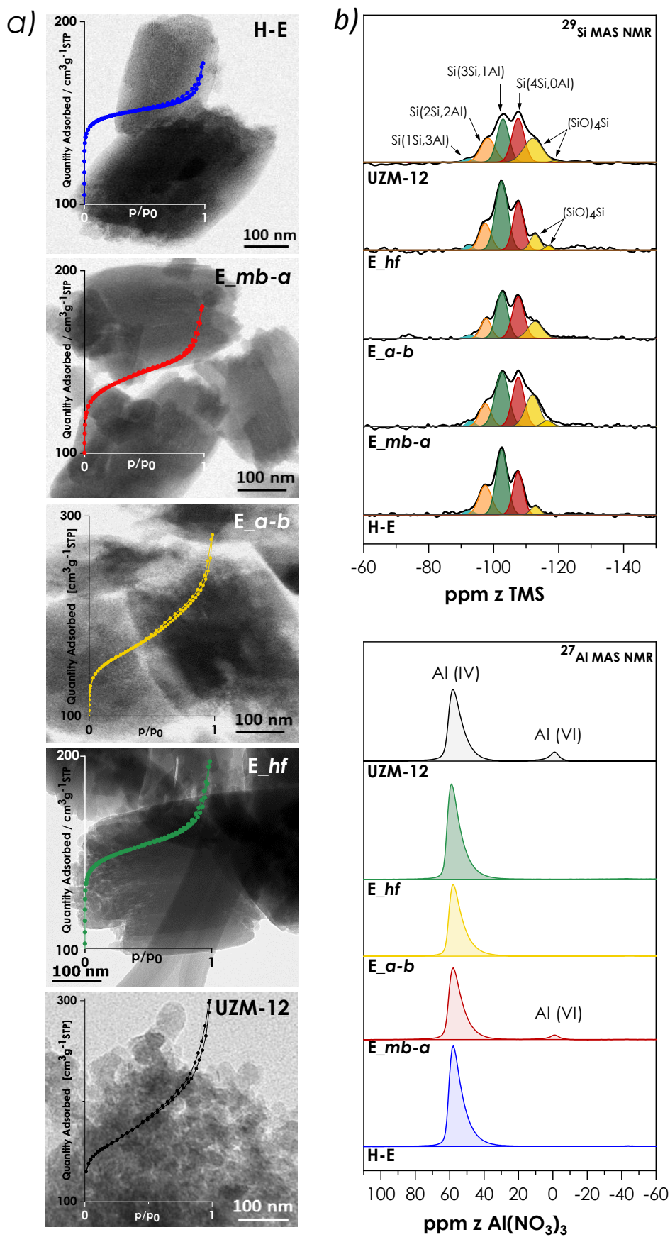
1 Fig. 2. (a) N_2 adsorption/desorption isotherms, STEM micrographs and (b) magic angle spinning NMR spectra of studied 2 samples.
