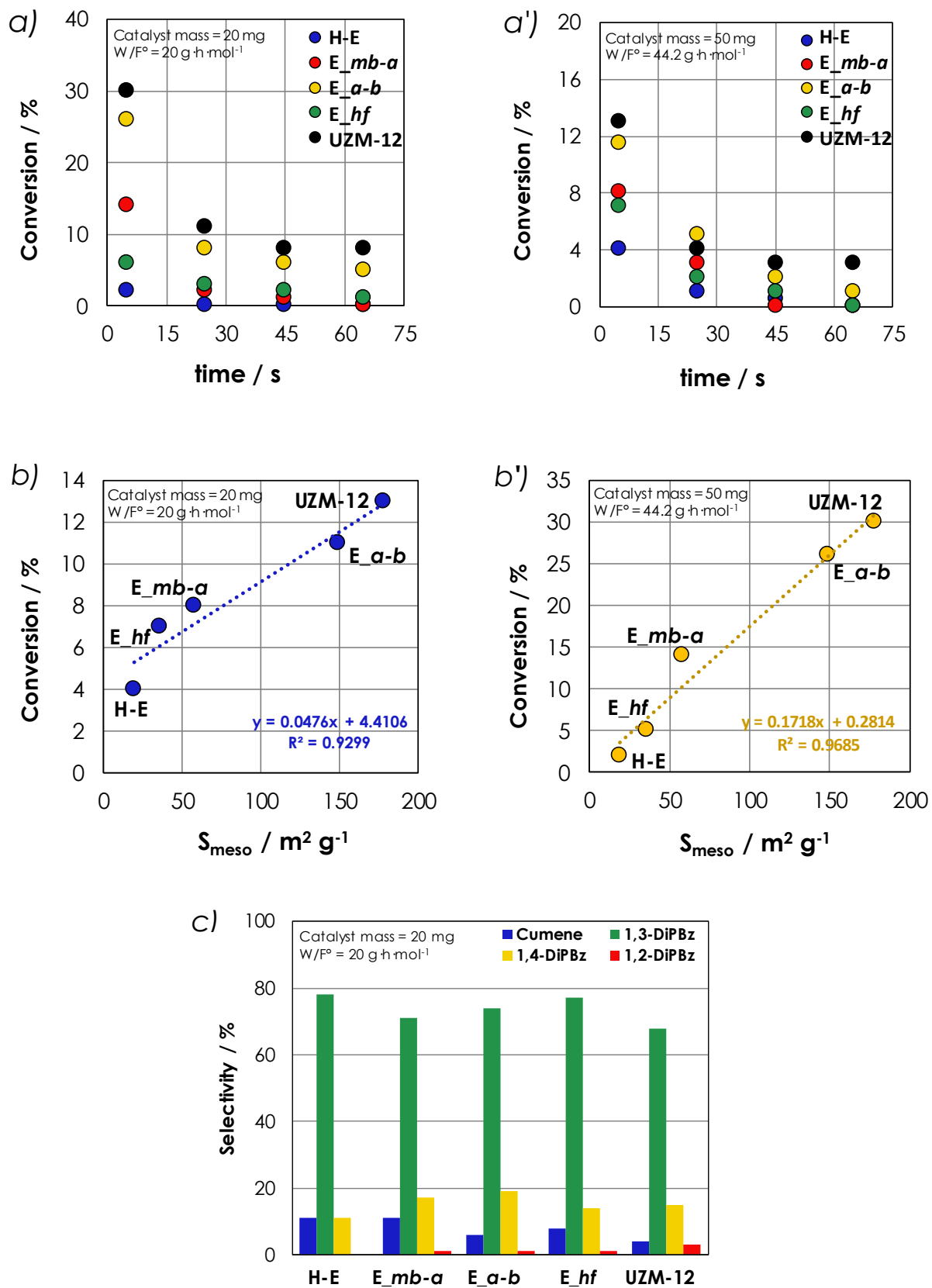
Fig. 4. (a) Conversion evolution in time in TiPBz dealkylation (b) conversions at short time on stream and a function of the mesopores surface area and (c) selectivity of the erionites studied in 1,3,5-trisopropylbenzene dealkylation at 20 \text{ g} \cdot \text{h} \cdot \text{mol}^{-1} .
