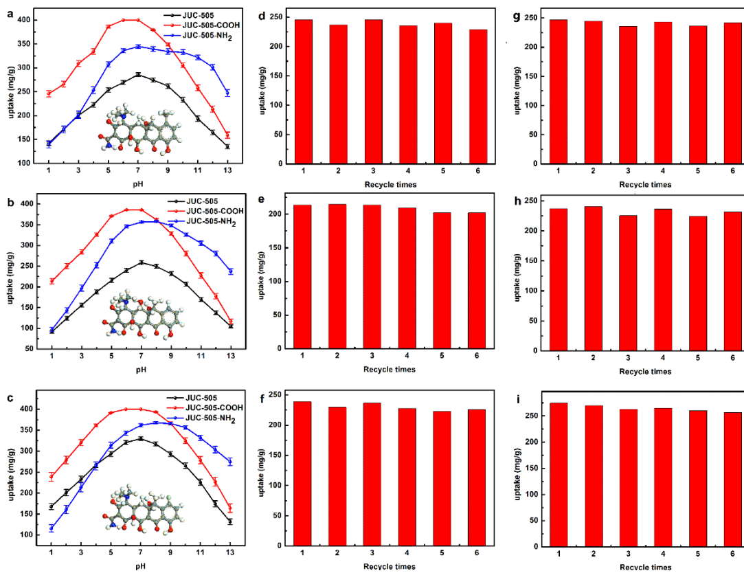
Figure 4 | Study of antibiotic uptakes. a-c , TCN, OTC and CTC uptakes at different pH (initial concentration = 200 mg/L, contact time = 72 h, sorbent dosage = 0.5 g/L, temperature = 298 K). Inset: molecular structure of TCN, OTC and CTC. O, red; N, blue; C, grey; H, white; Cl, cyan. d-f , Recycling test of TCN, OTC and CTC uptakes of JUC-505-COOH at pH = 1. g-i , Recycling test of TCN, OTC and CTC uptakes of JUC-505-NH 2 at pH = 13.
