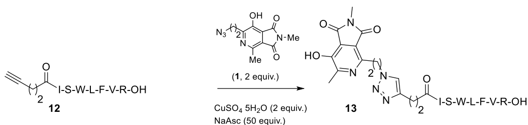
Scheme 2. Labeling of alkyne-oligopeptide 12 with azide 1 .
