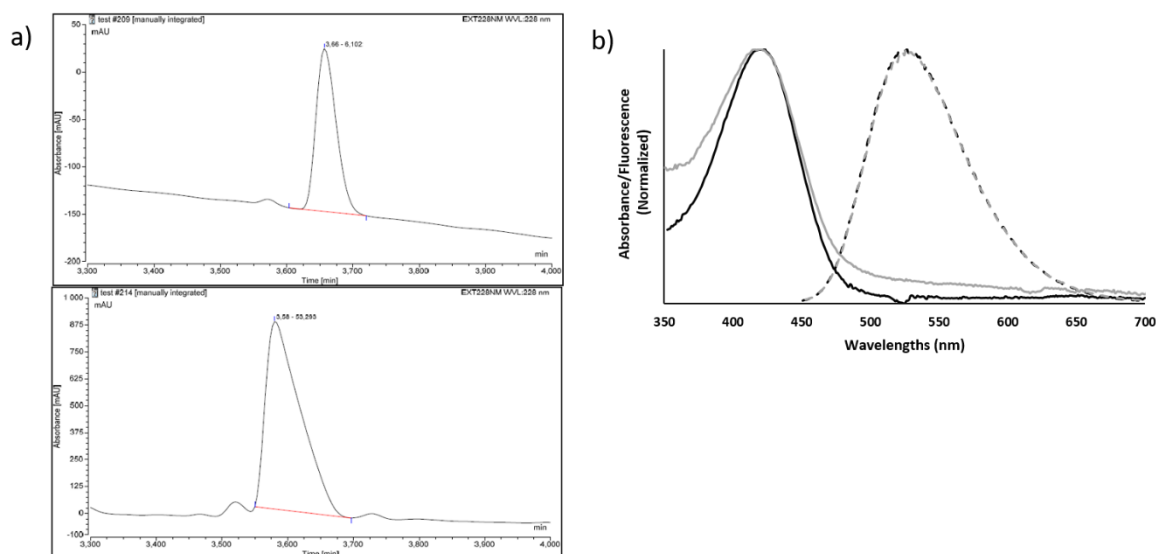
Figure 3. Green-fluorescence labeling of peptide 12 . a) RP-HPLC chromatogram of peptide-alkyne 12 (top) and labeled peptide 13 after 30 min reaction (bottom). b) Normalized absorption (solid line)
