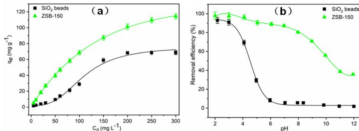
Figure 5. Aniline adsorption capacity(a) and Impact of pH on the aniline adsorption (b) of SiO 2 and ZSB-150 beads (adsorption time: 12 h, adsorption temperature: 25 °C, Co: 20 mg L -1 , adsorbent: 1 g L -1 ).
